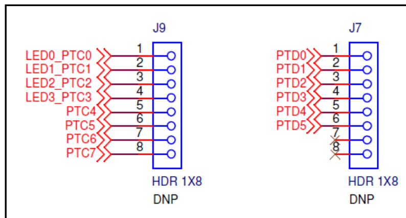
Figure 10 FTM2 and PWT pin assignment
