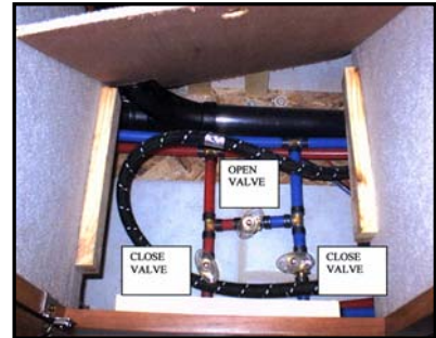
Figure 11-8. Water Heater Bypass System
