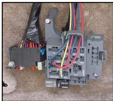
Figure 7-10. Fuse Blocks
