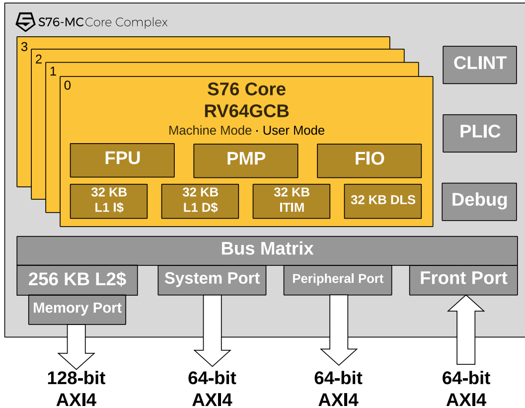
Figure 1: S7 Series Block Diagram
