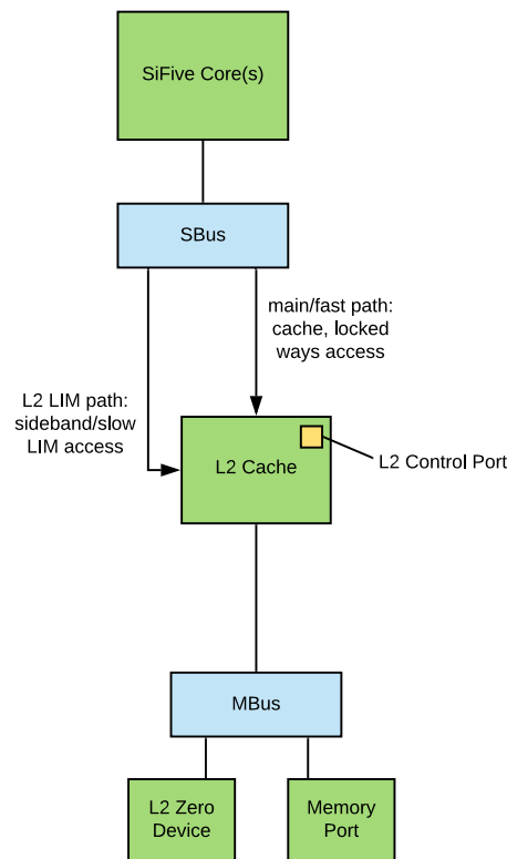
Figure 106: Difference between L2 LIM and L2 Zero Device
