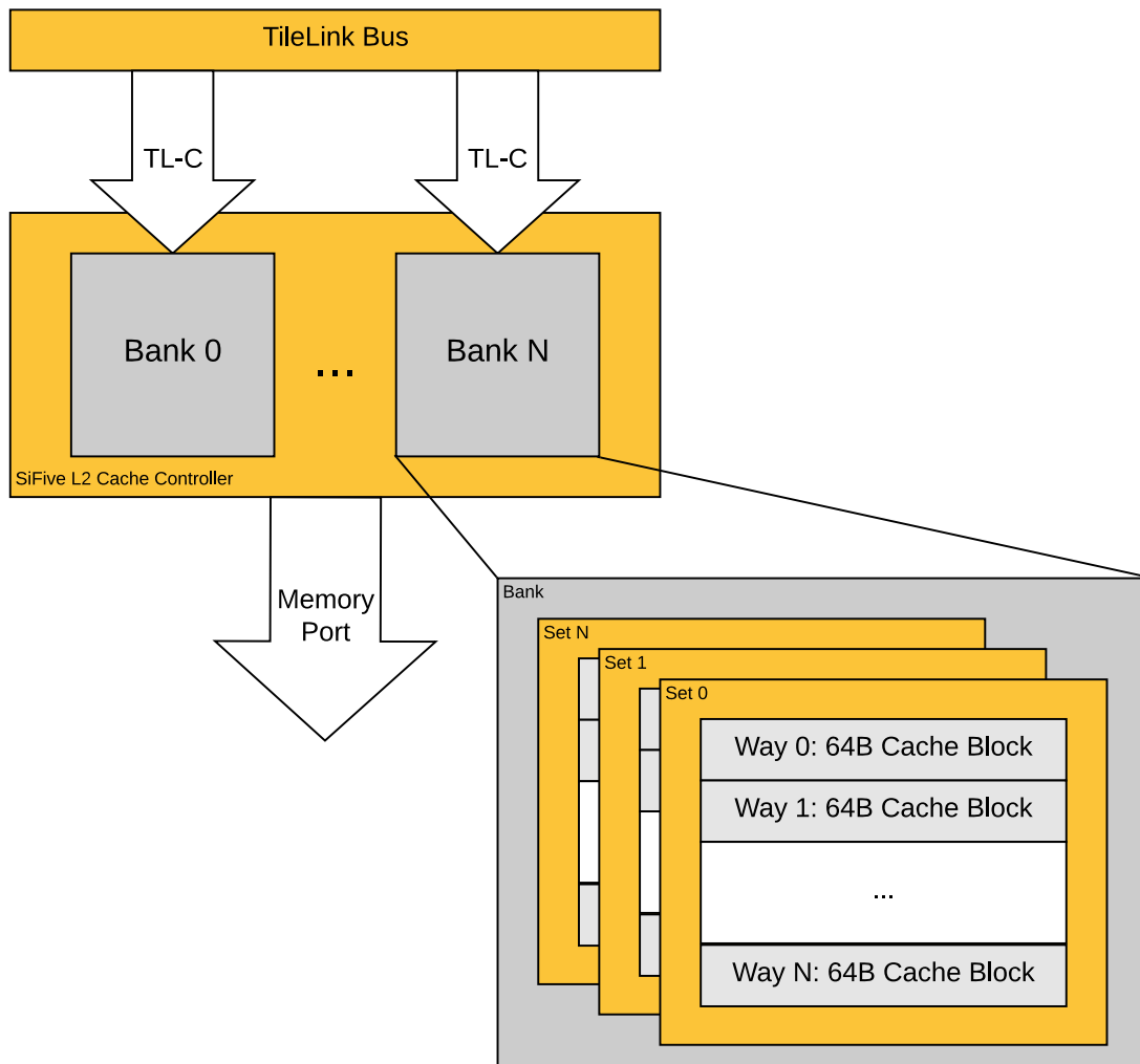
Figure 104: Organization of the SiFive L2 Cache Controller
