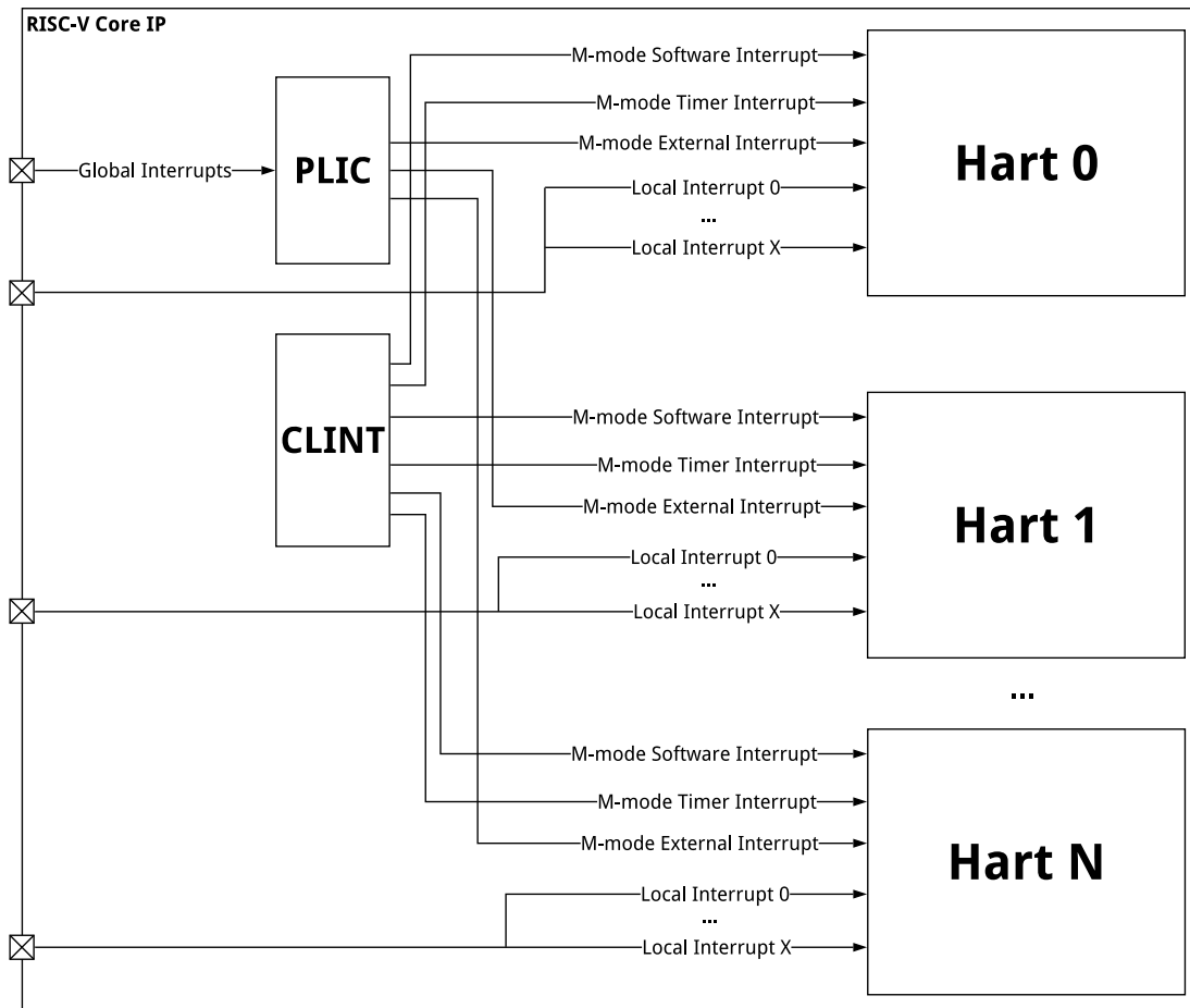
Figure 98: S76-MC Core Complex Interrupt Architecture Block Diagram
