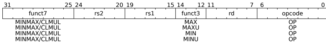
Figure 83: Comparison Instructions
