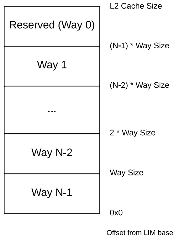
Figure 105: Mapping of L2 Cache Ways to L2 LIM Addresses
