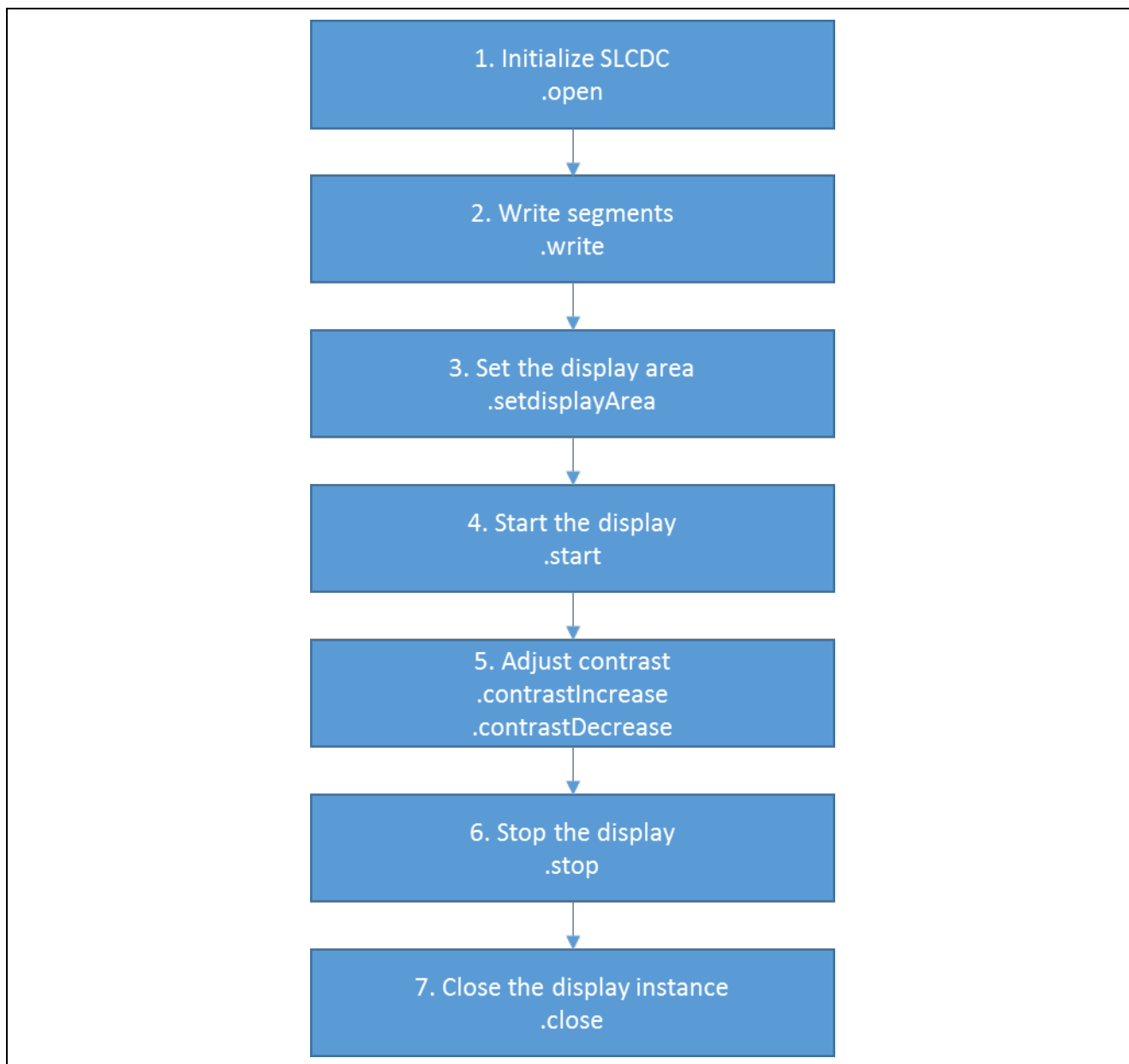
Figure 3 Flow Diagram of a Typical Segment LCD HAL Module Application
