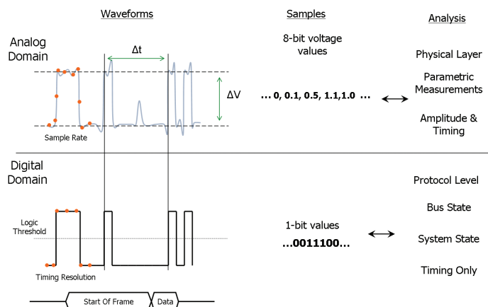
Figure 1. Analog and digital measurement differences.
