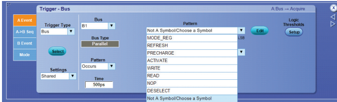
Figure 3. Triggering with user-definable Bus definitions.
