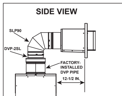
Figure 3.6 PVLP-SLP Minimum Horizontal Footprint (PRIMO48, PRIMO60, PRIMO72)
