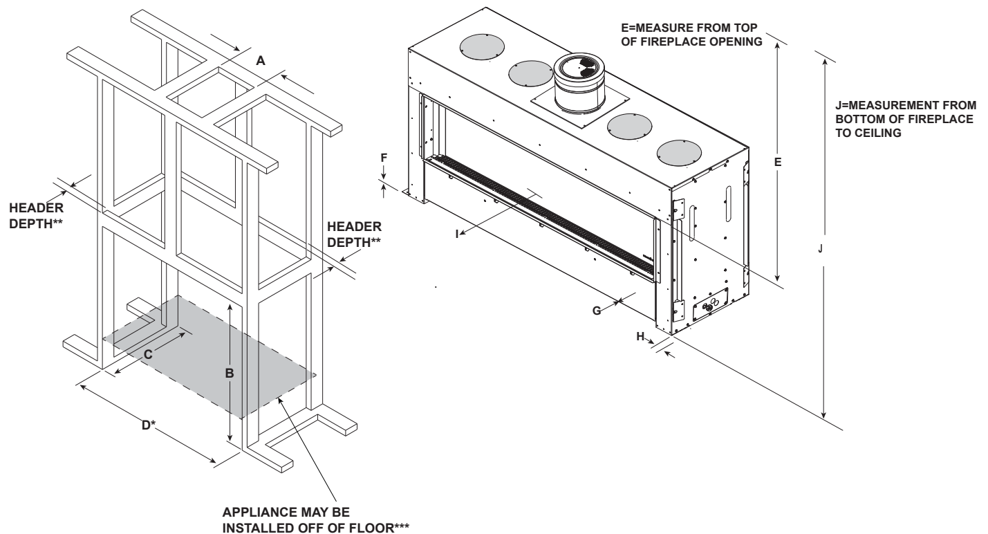
MINIMUM FRAMING DIMENSIONS* (See-Through Models)
