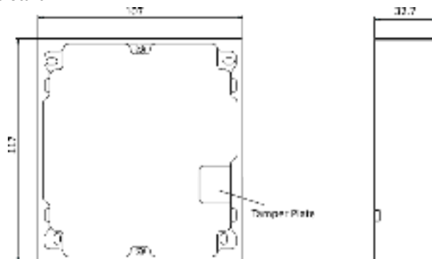
Figure 3-2 Mounting Frame
