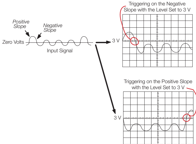
Figure 35. Positive and negative slope triggering.
