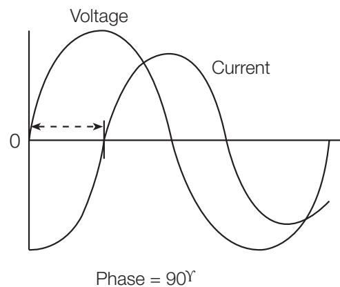
Figure 10. Phase shift.
