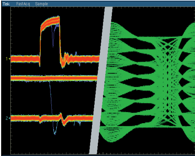
Figure 15. Some DPOs can acquire millions of waveform in just seconds, significantly increasing the probability of capturing intermittent and elusive events and revealing dynamic signal behavior.
