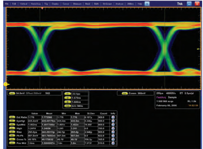
Figure 7. 622 Mb/s serial data eye pattern.
