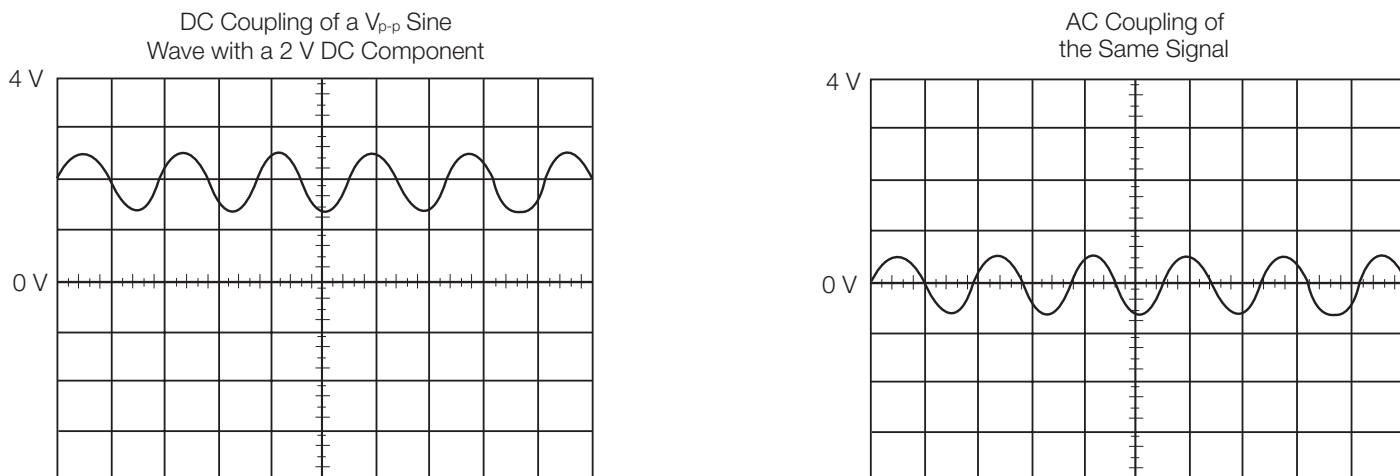
Figure 21. AC and DC input coupling.
