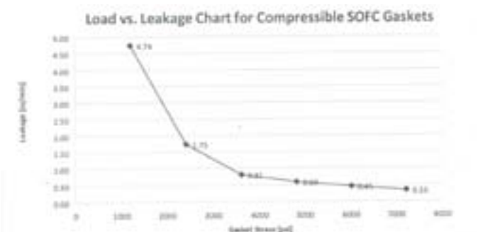
Fig. 3a Compressive load vs. leakage for a talc-based gasket
