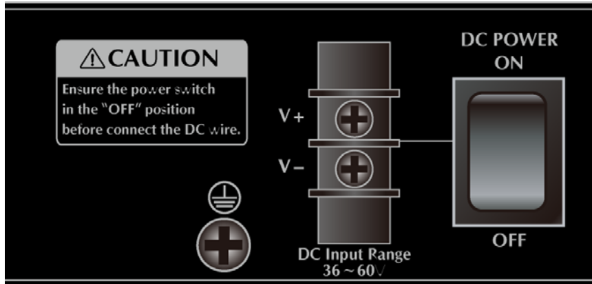
Figure 2-1-23 Rear Panel of GS-5220 PoE series Redundant Power Models
