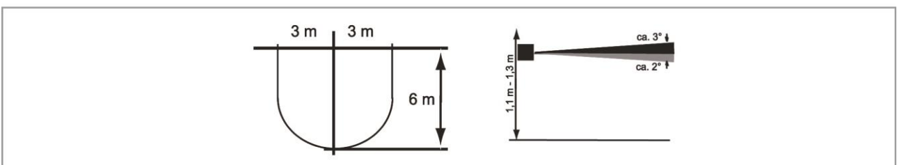
Fig. 40 Detection range
