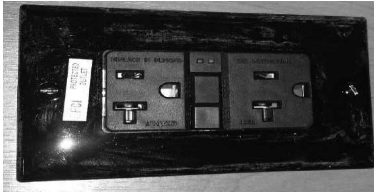
Figure 9-5 GFCI Receptacle
