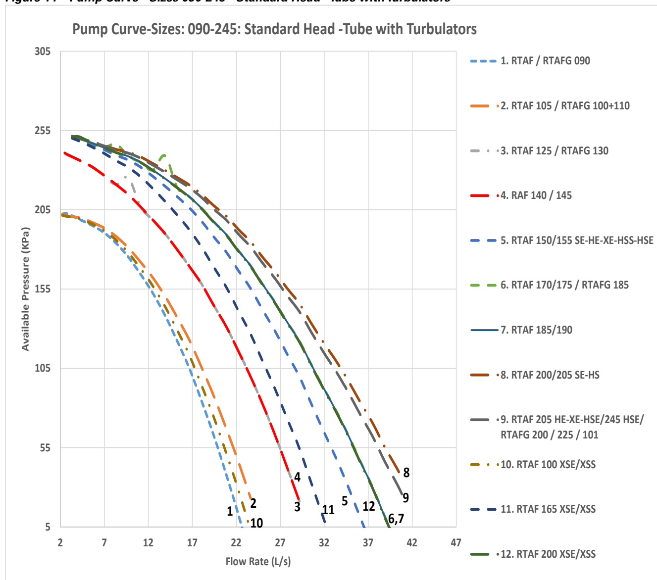
Figure 14 – Pump Curve - Sizes 090-245 - Standard Head - Tube with Turbulators
