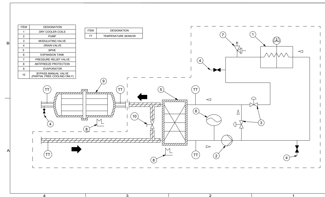
Figure 24 – Flow chart - Free cooling - Glycol free version
