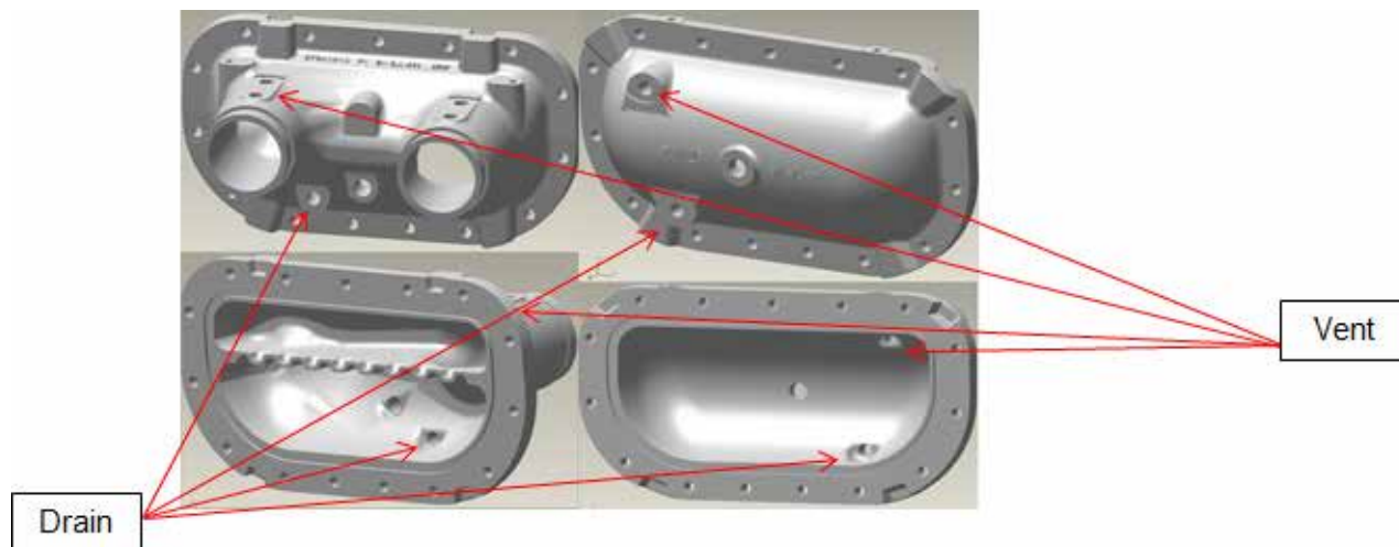
Figure 4 – Drain and vent position on evaporator
