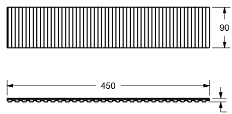
Figure 2 – Isolator pads
