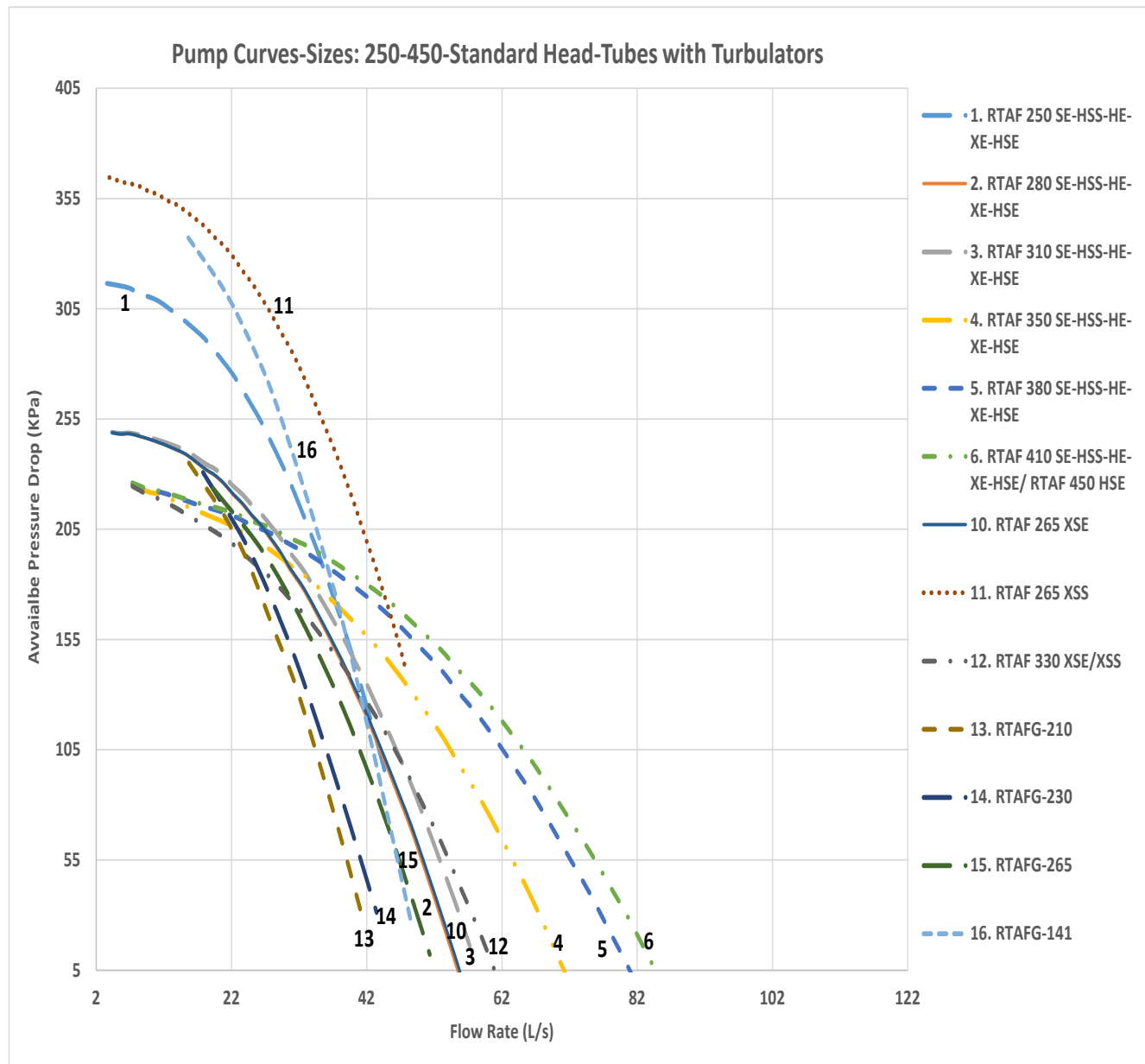
Figure 16 – Pump Curve - Sizes 250 - 450 - Standard Head - Tubes with Turbulators
