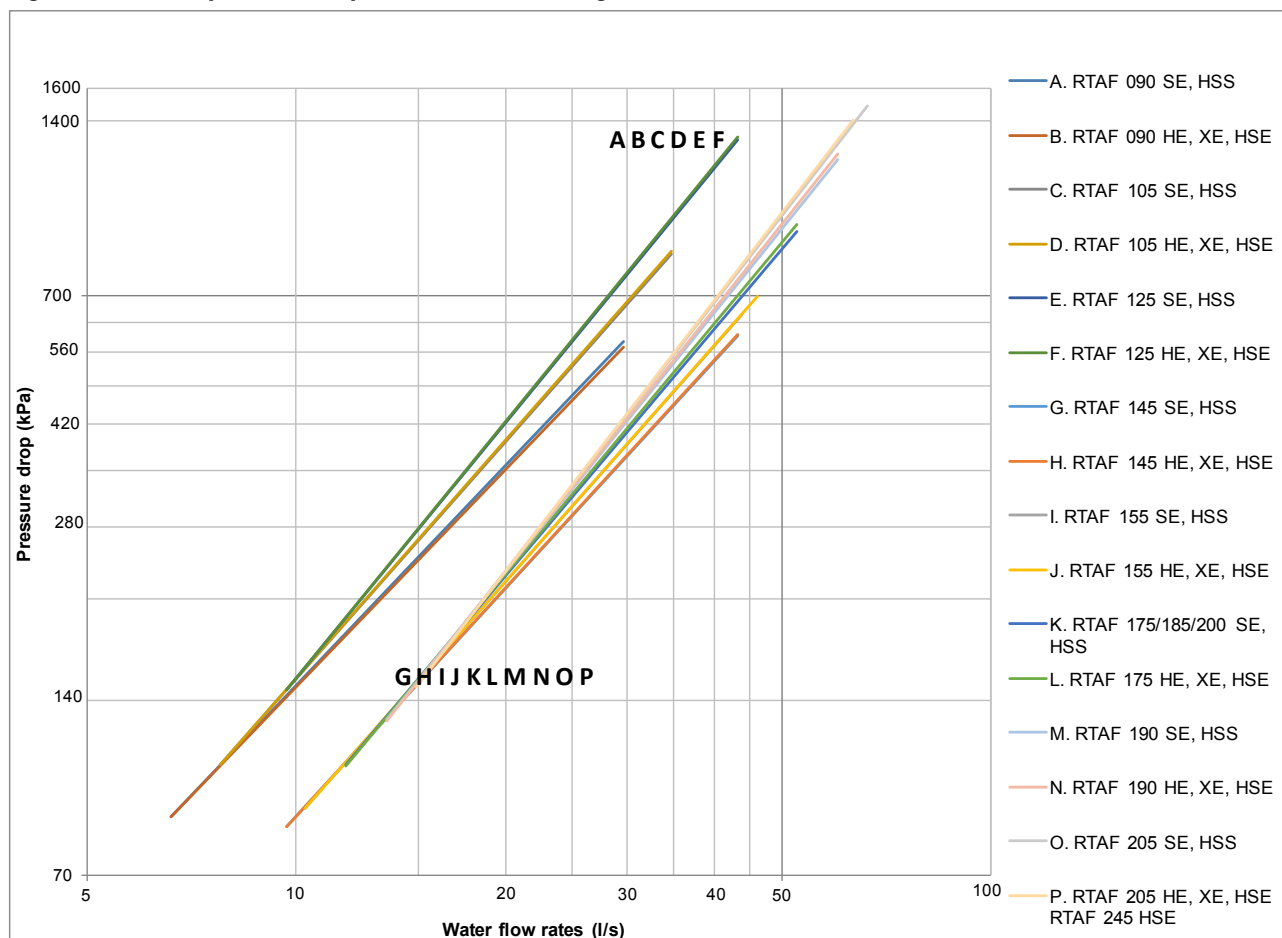
Figure 25 – Water pressure drop - Partial Free-Cooling - Sizes 090-245
