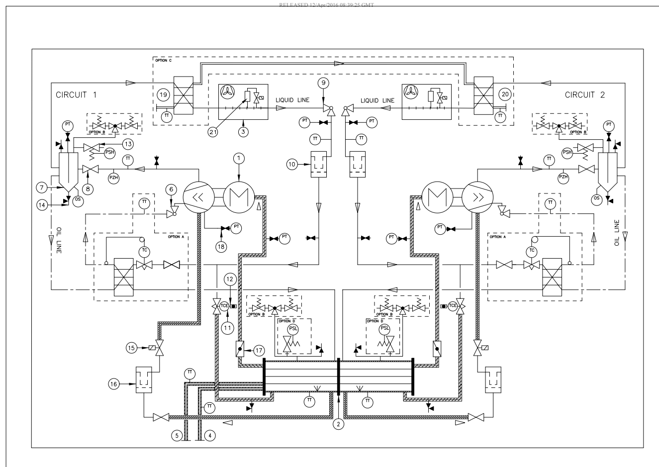
Figure 33 – Example of Typical Refrigerant System Schematic & Oil Lube Circuit Schematic
