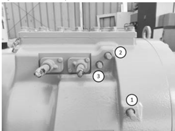
Figure 40: GP4 Compressor
