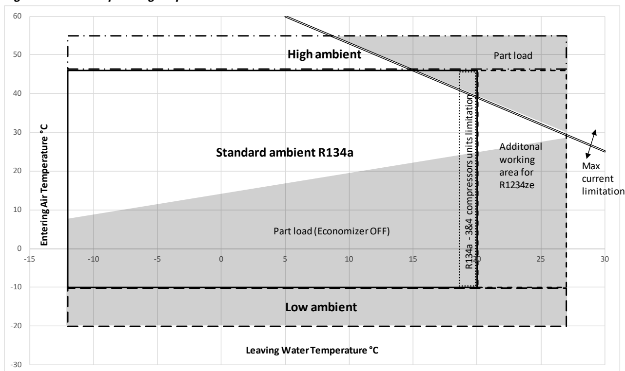
Figure 35 – RTAF Operating Map
