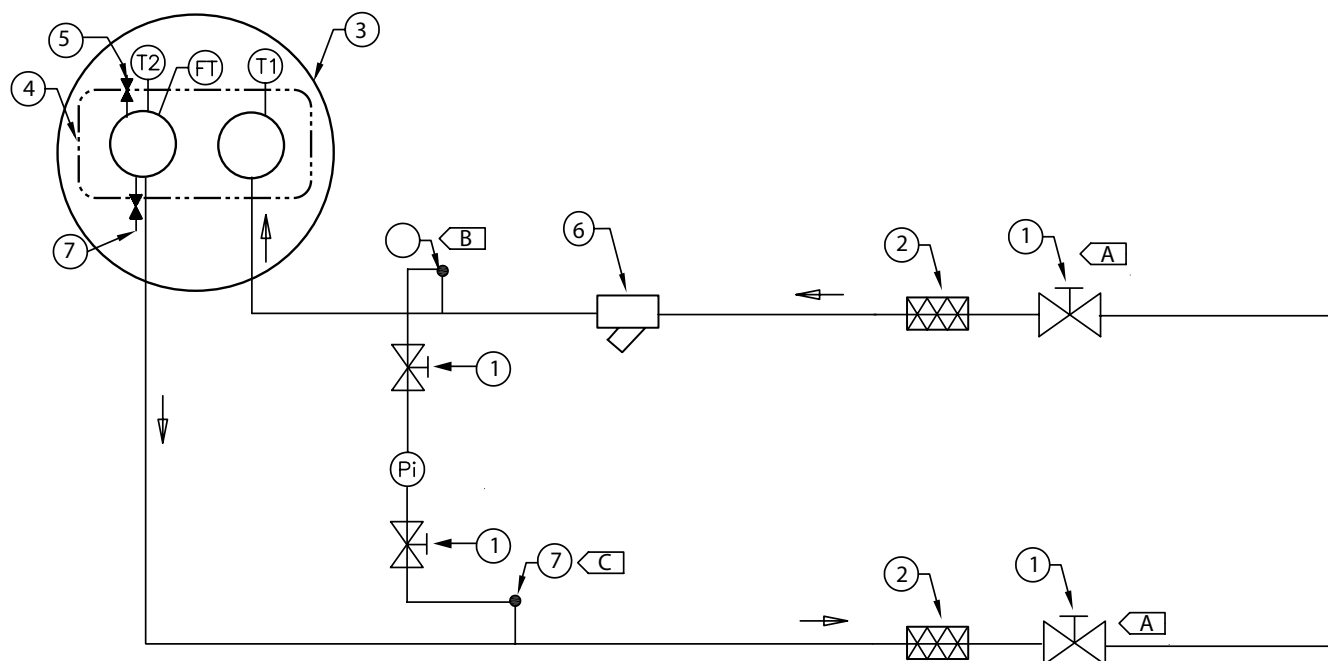
Figure 3 – Typical RTAF evaporator water piping
