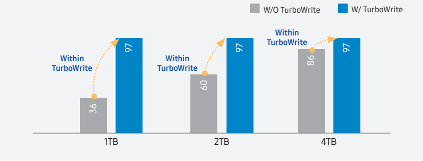
Figure 6. Random read performance comparisons (in KIOPS)
