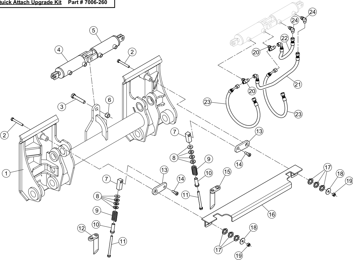
Power Quick Attach Upgrade Kit Part # 7006-260
