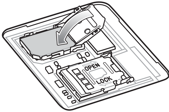
Figure 25 Close the SIM Card Door
