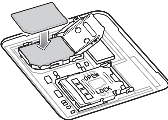
Figure 6 Place SIM Card in Holder
