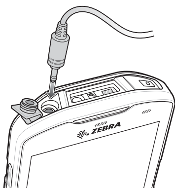
Figure 164 Audio Adapter Installation
