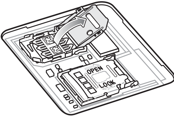
Figure 5 Lift the SIM Card Holder
