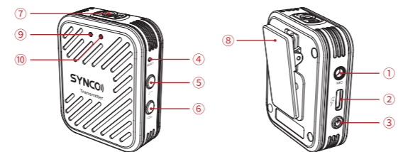
TX Transmitter
