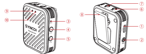
RX Receiver
