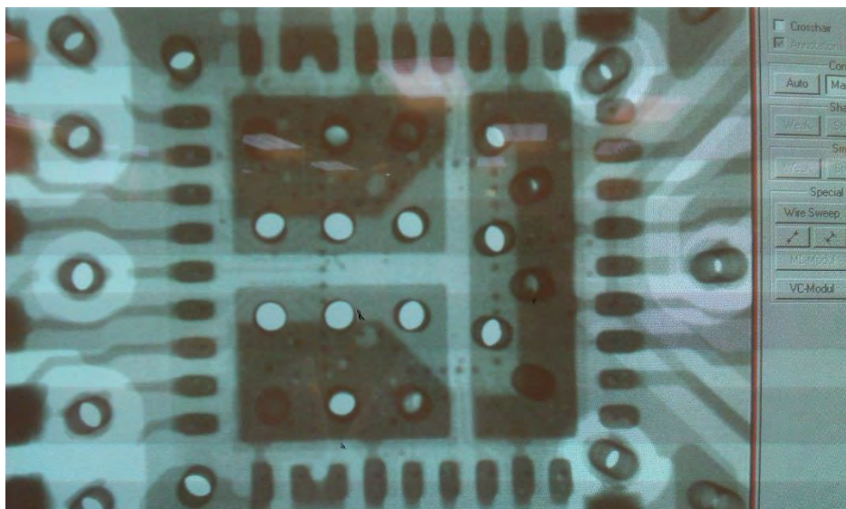
Fig 19. X-ray of soldered device
