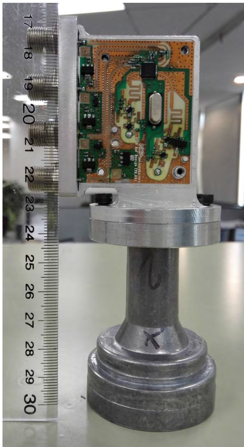
Fig 8. NXP Quad Reference LNB
