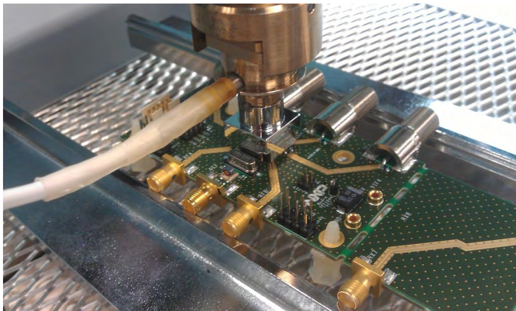
Fig 16. soldering process 2
