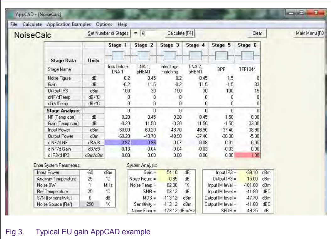
Fig 3. Typical EU gain AppCAD example In this Noise/Gain budget example for a 55dB Gain LNB, based on Rogers material. We assume two frequently used pHEMT devices are applied as LNA1/LNA2 stages. Gain mode for TFF1044 is medium, values applied are typical (overall typical Gain is 54 dB, NF is 0.85 dB).
