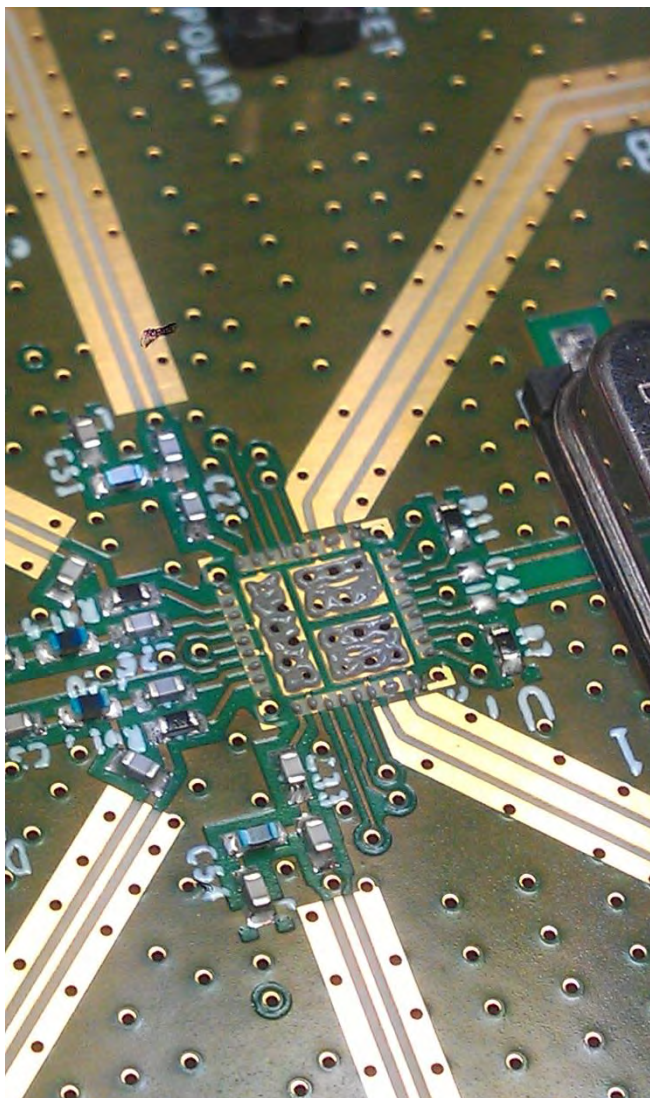
Fig 13. Solder paste applied
