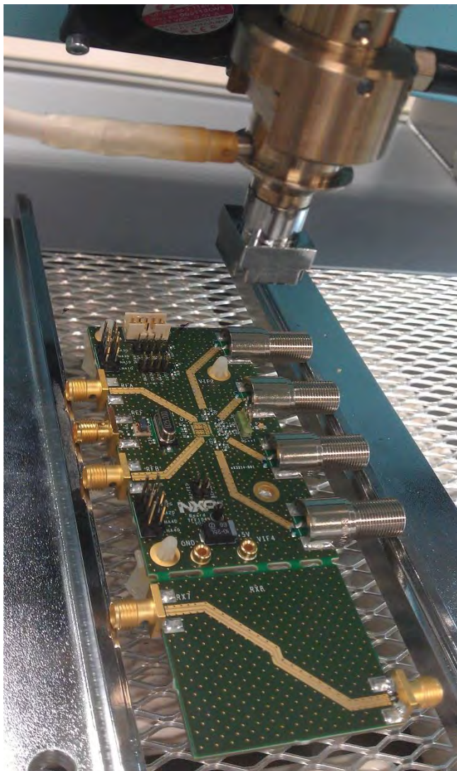
Fig 15. soldering process 1
