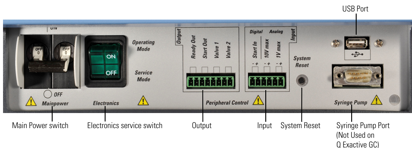
Figure 3-4. Power panel
