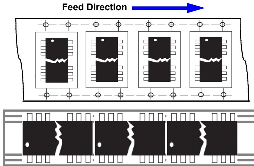
Figure 16. HSOP orientation in tube and tape and reel
