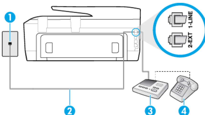
Figure B-11 Back view of the printer
