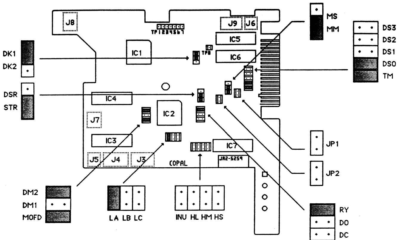
Figure 4-1C M2552K Revision 1 Circuit Card - Jumper Locations
