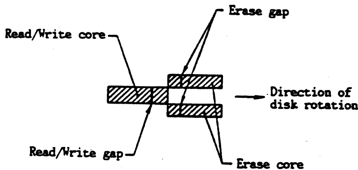
Figure 3-2 Tunnel Erase Type Read/Write Head
