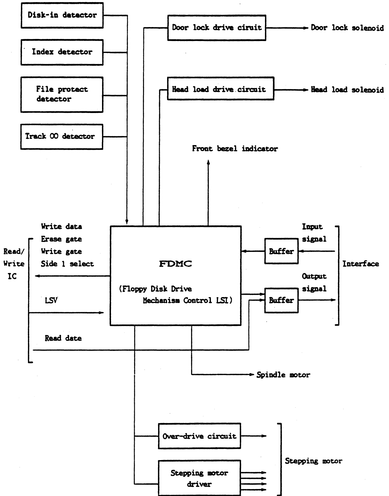
Figure 3-6 Control Circuits
