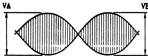
Figure 4-11 Lobe Pattern for Track Alignment
