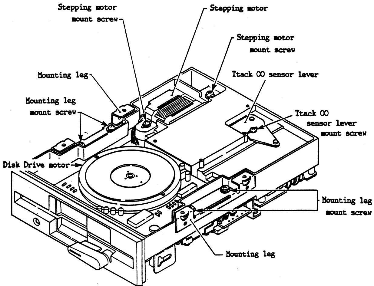
Figure 5-3 Bottom View of Disk Drive
