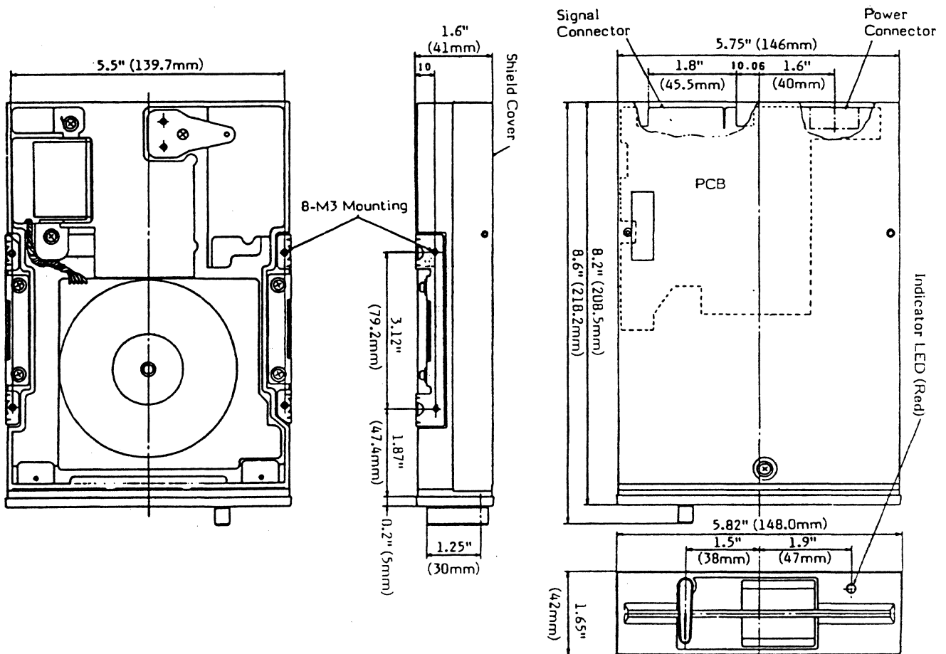
Figure 2-1 External Outline Drawing of Disk Drive
