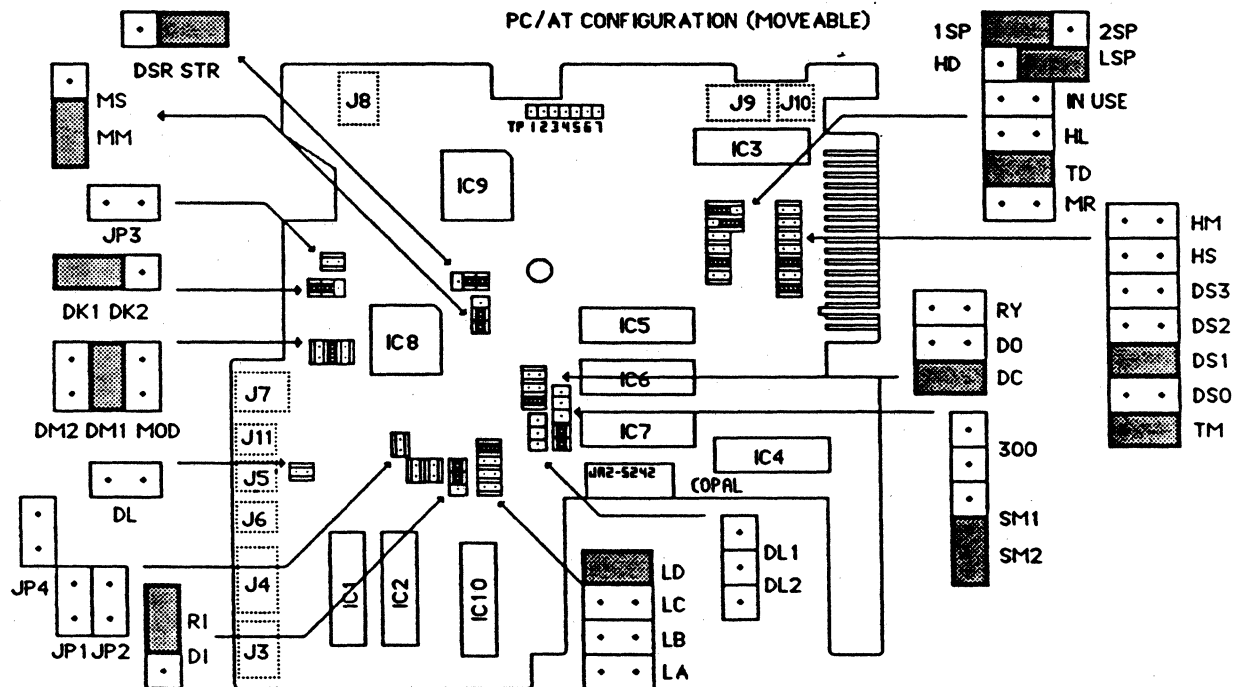
Figure 4-1A M2553K/54K Revision 2 Circuit Card - Jumper Locations
