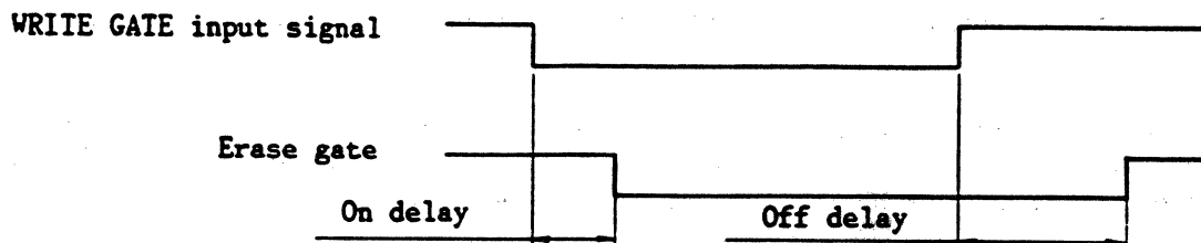
Figure 3-11 TP6 Typical Erase Gate Waveform
