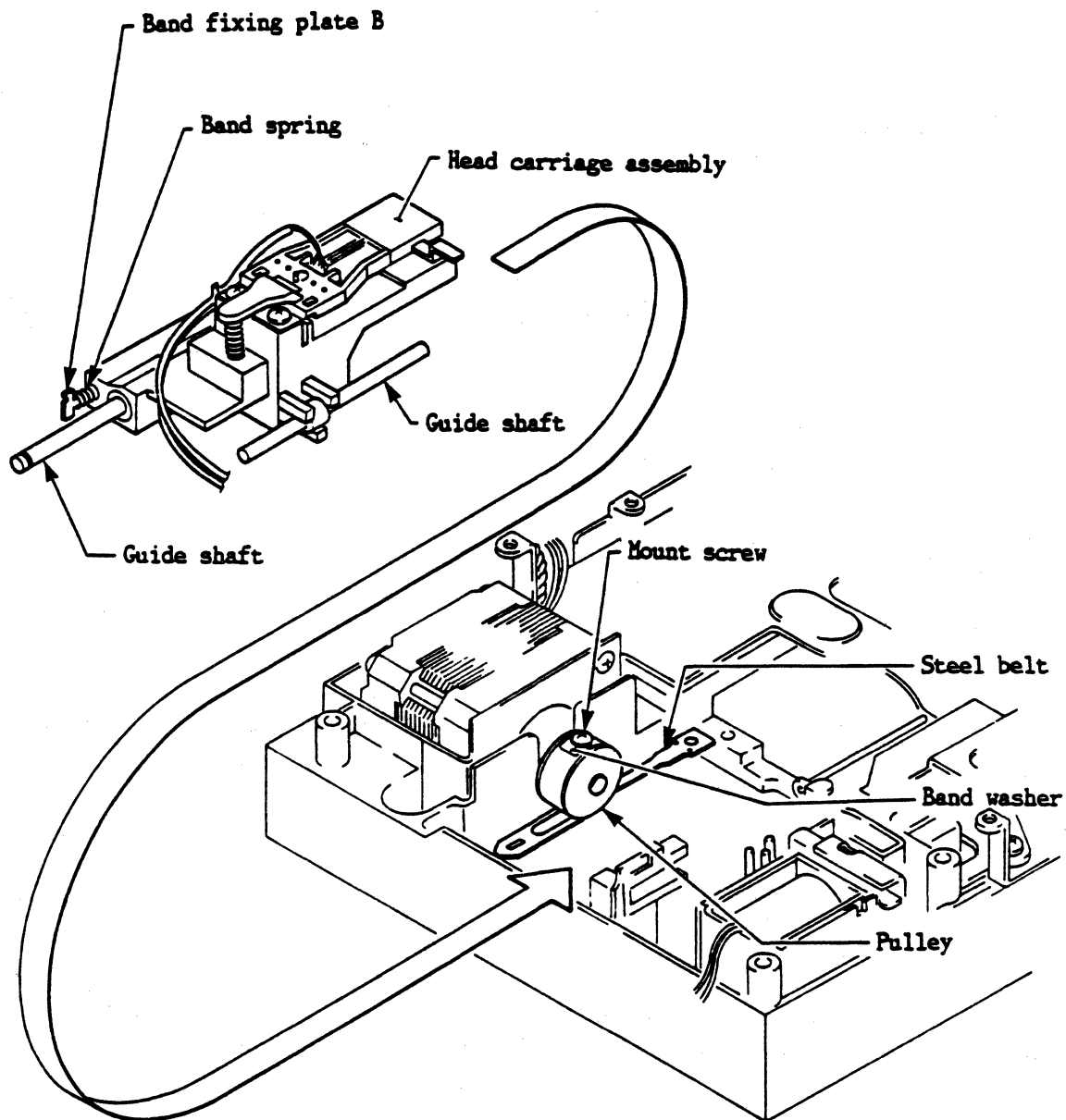
Figure 4-23 Head Carriage Assembly Replacement
