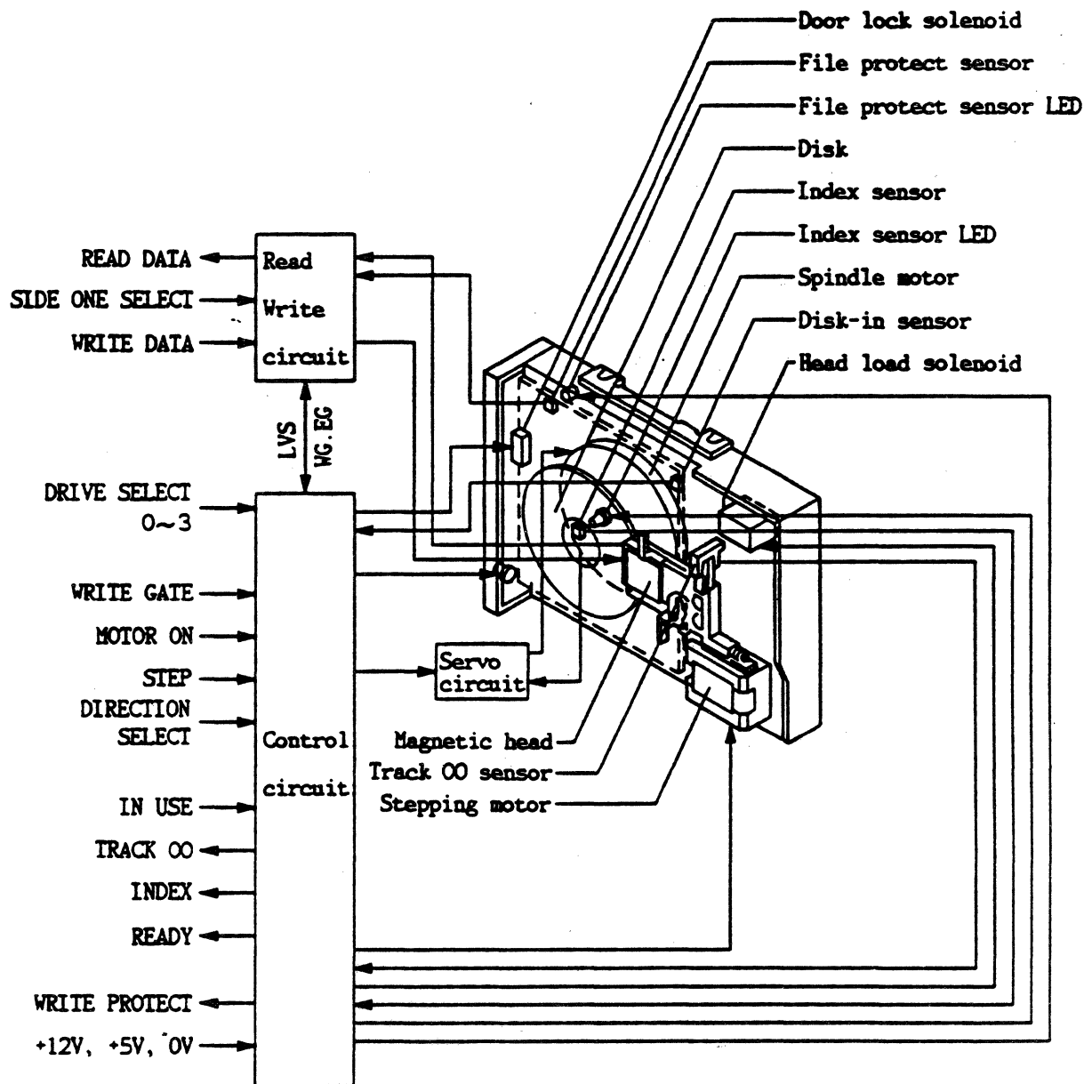
Figure 3-1 Overall Block Diagram
