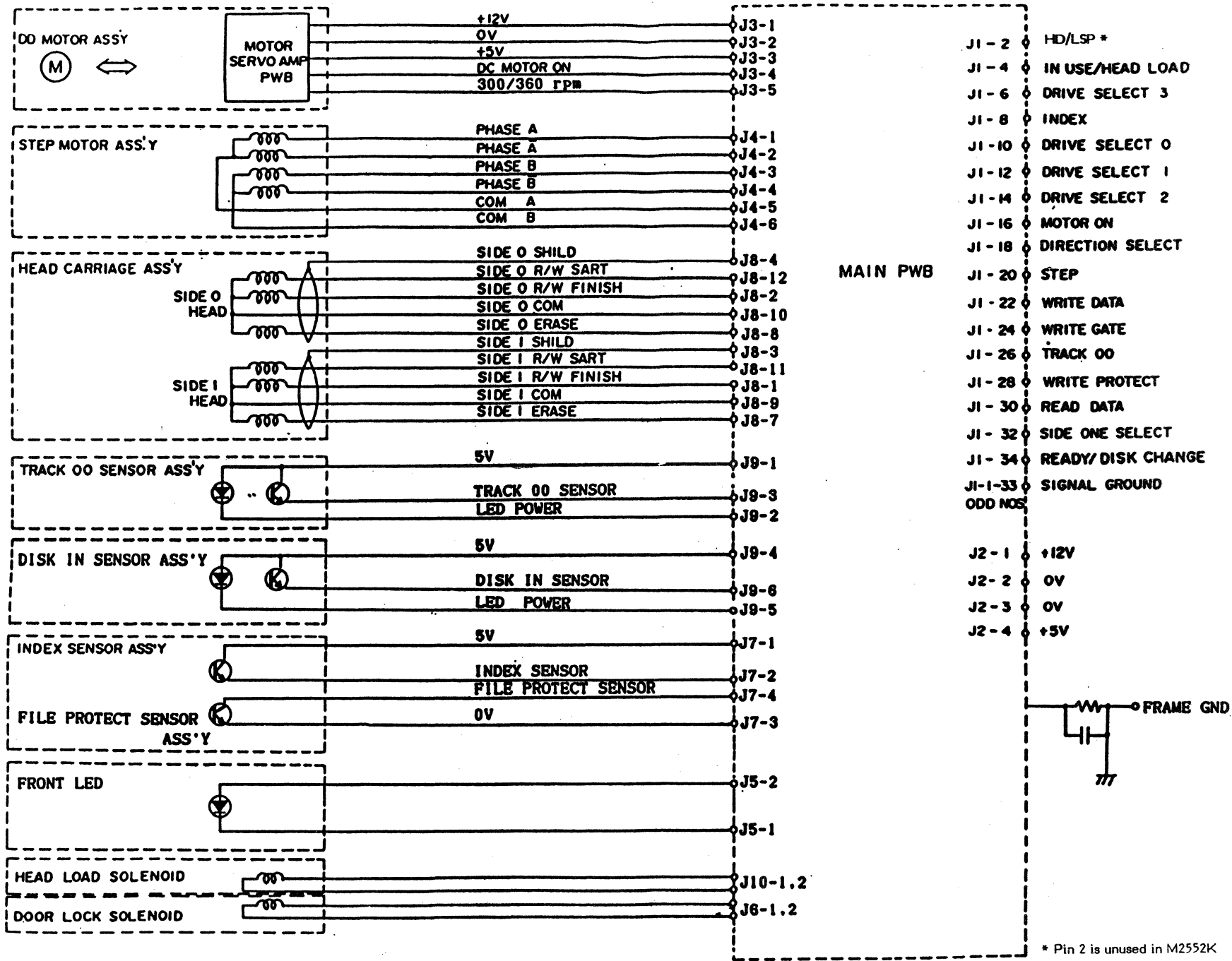
Figure 5-9 Interconnect Diagram
