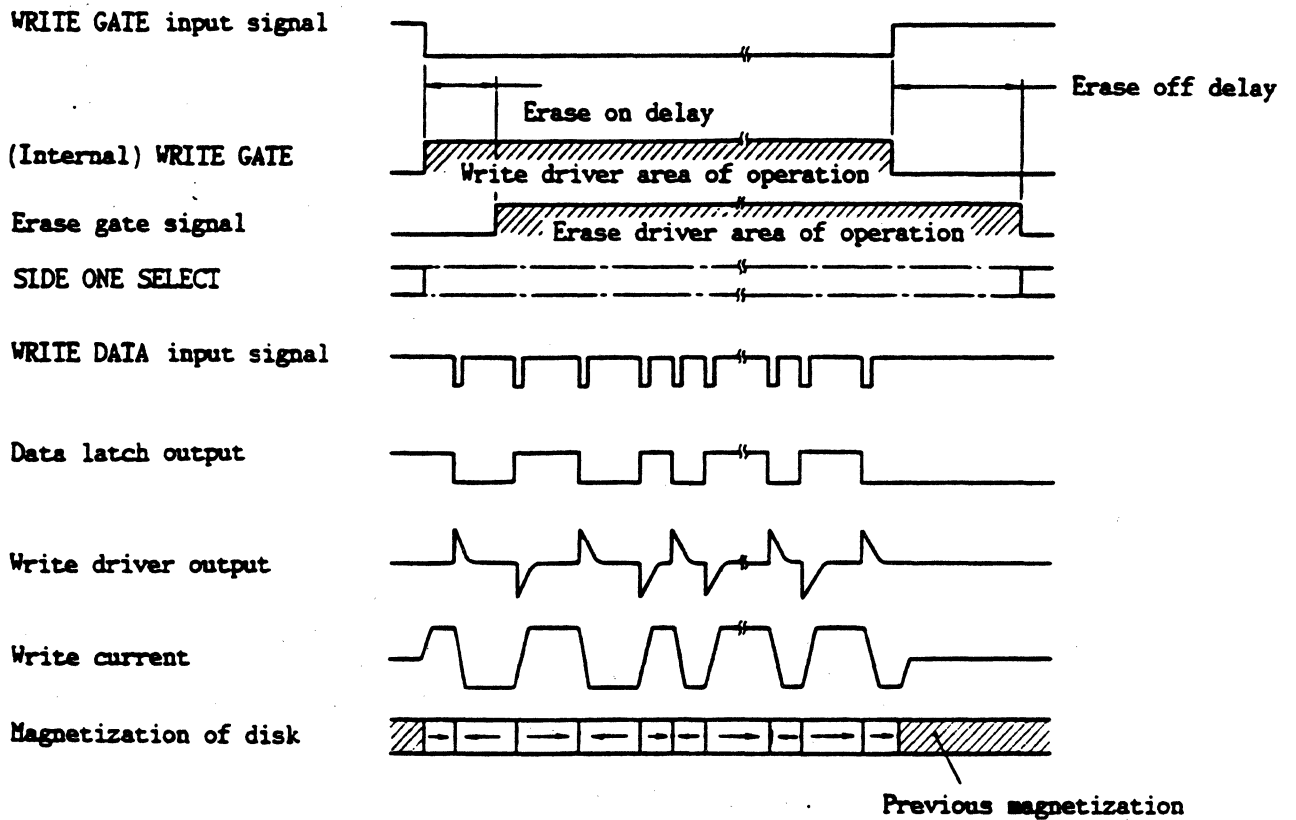
Figure 3-5 Typical Write Circuit Waveforms
