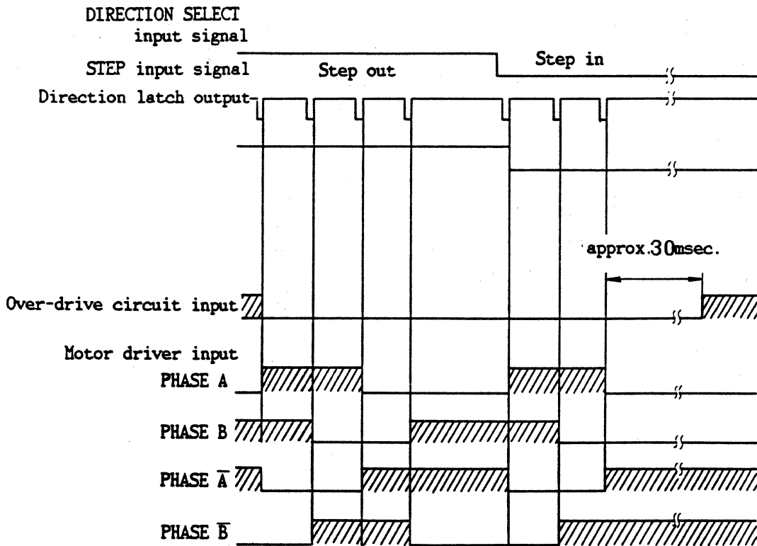
Figure 3-7 Typical Stepping Motor Control Circuit Waveforms
