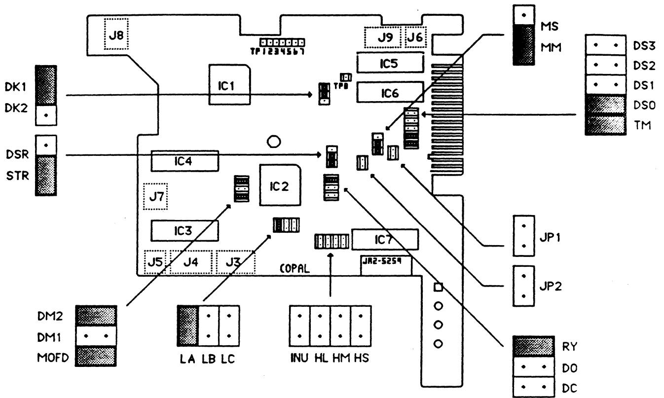
Figure 5-6 M2552K Revision 1 Circuit Card Layout
