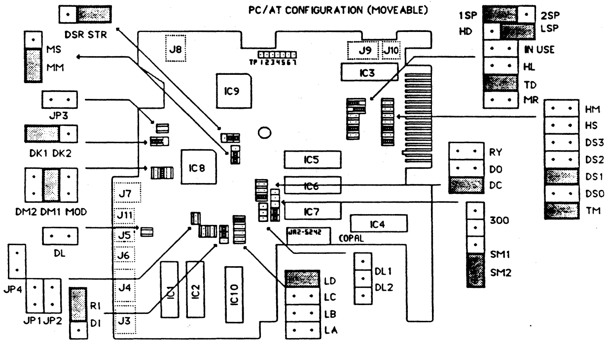
Figure 5-7 M2553/54K Revision 2 Circuit Card Layout
