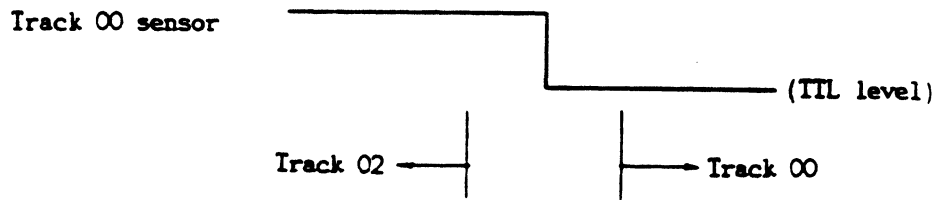
Figure 3-12 TP7 Track 00 Detect Waveforms
