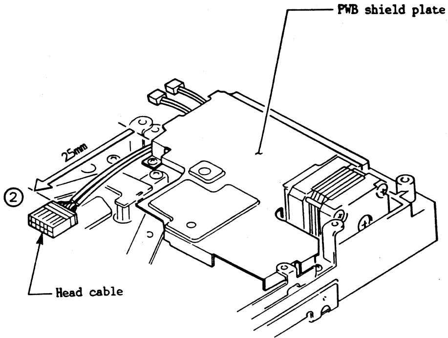
Figure 4-24B Head Cable Routing
