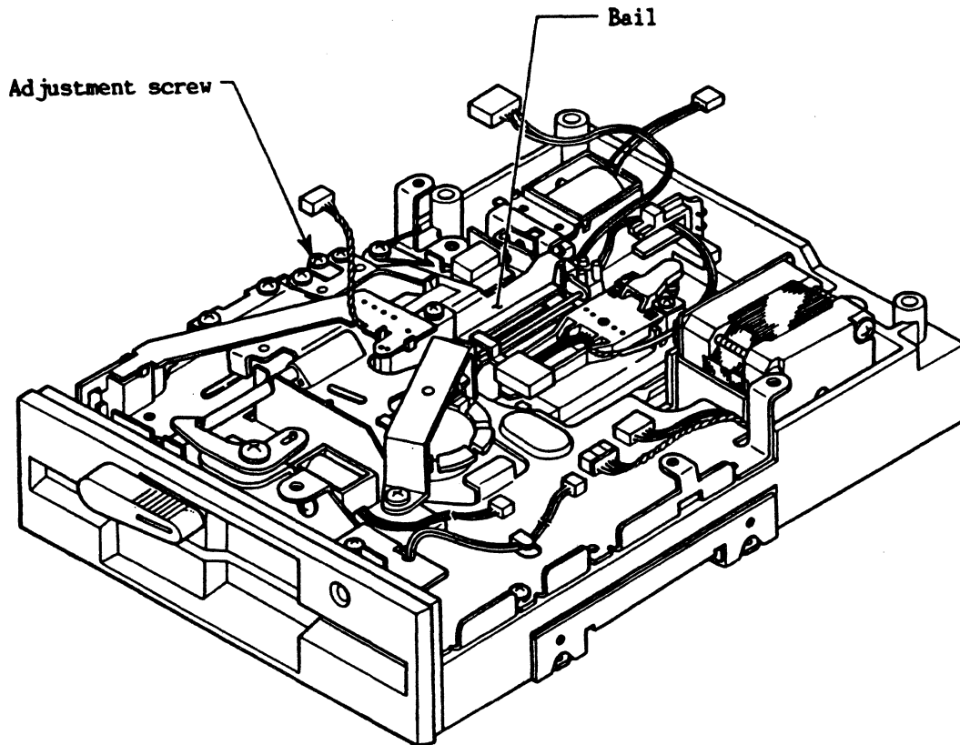
Figure 4-5 Bail Adjustment
