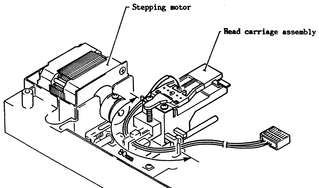
Figure 4-24A Head Cable Routing
