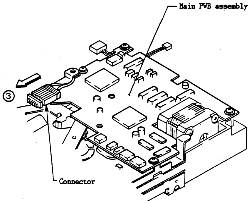
Figure 4-24C Head Cable Routing
