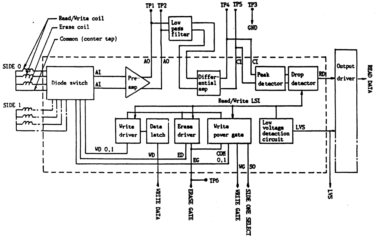
Figure 3-3 Read/Write Circuits
