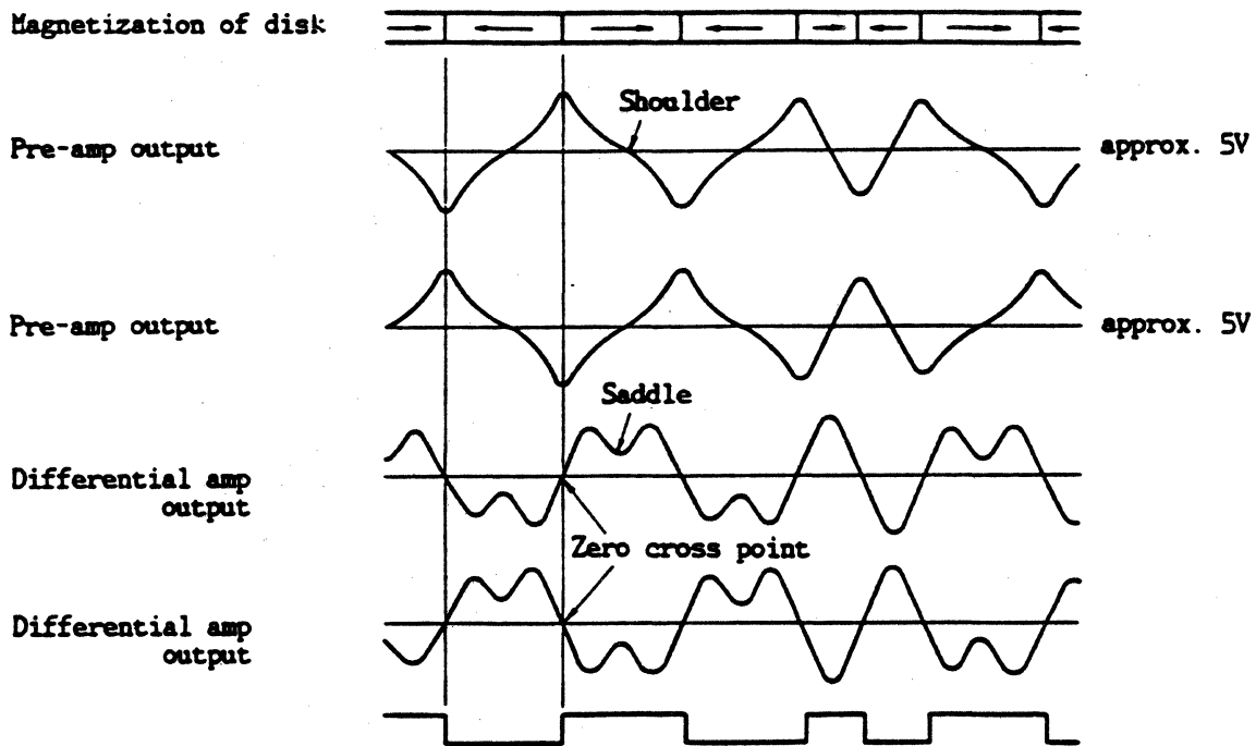
Figure 3-4 Typical Read Circuit Waveforms
