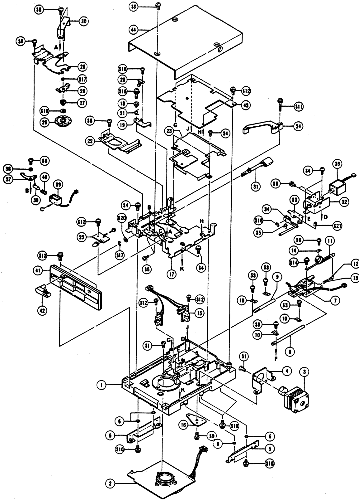
Figure 5-5 Exploded View Drawing
