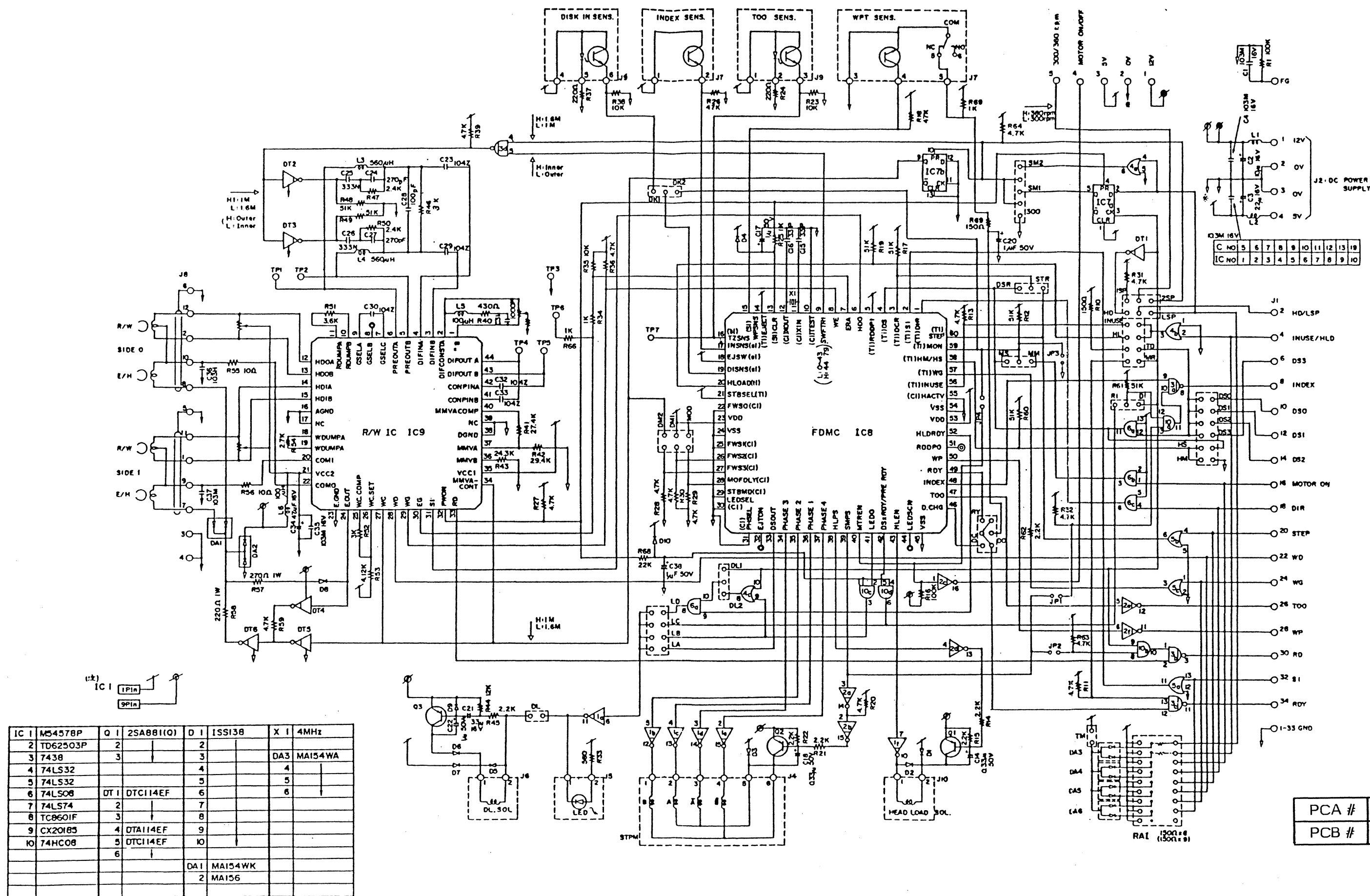
Figure 5-11 M2553K and M2554K Revision 2 Schematic Diagram
