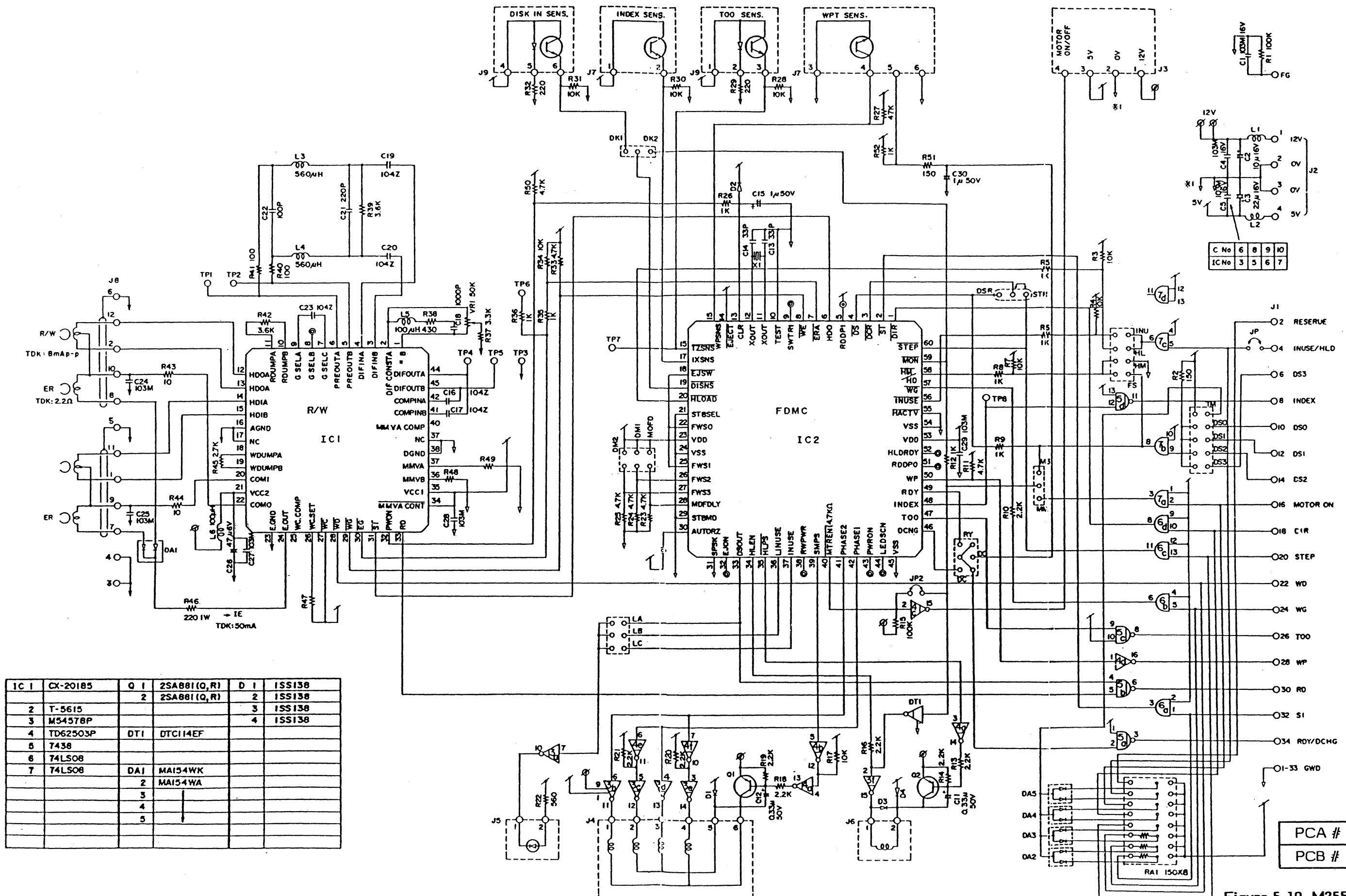
Figure 5-10 M2552K Revision:1 Schematic Diagram
