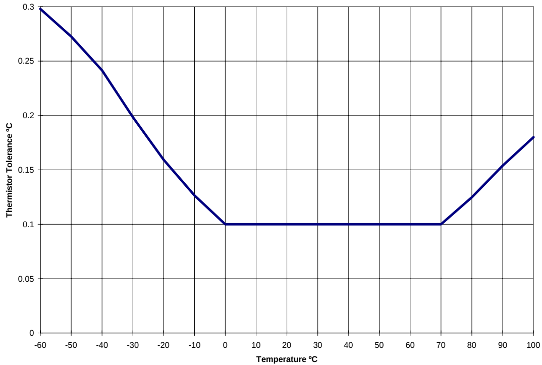
FIGURE 3.4-1. Thermistor Tolerance
