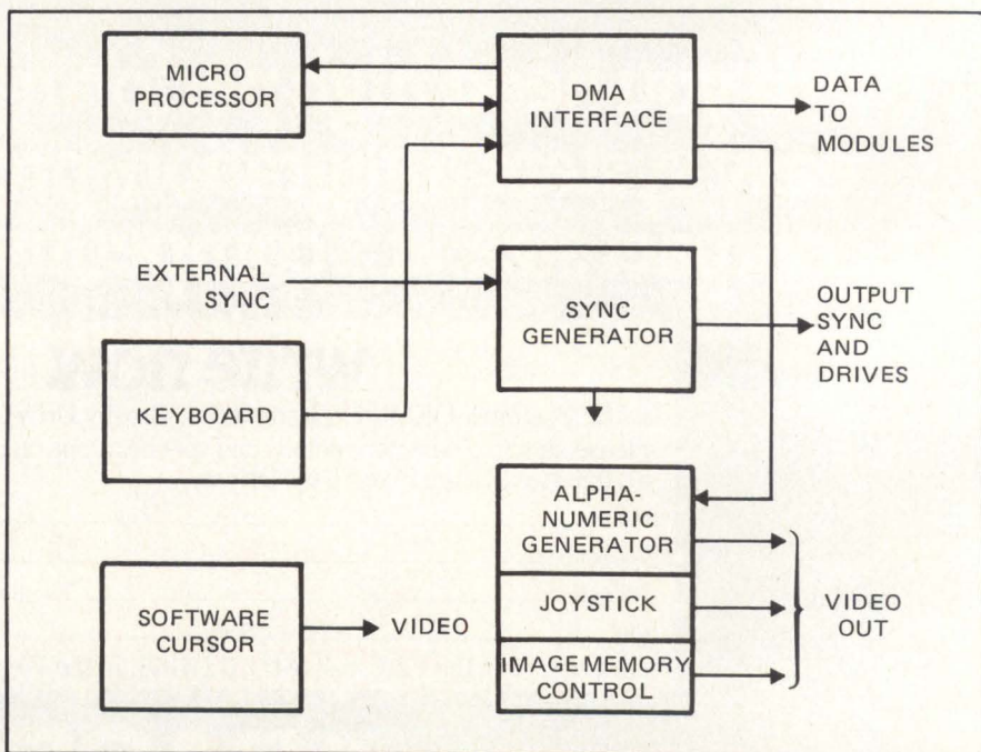
Figure 2: Core Subsystem contains the IDEX real-time bus switcher.
