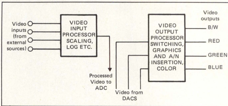
Figure 1: Analog Processor handles live incoming video.
