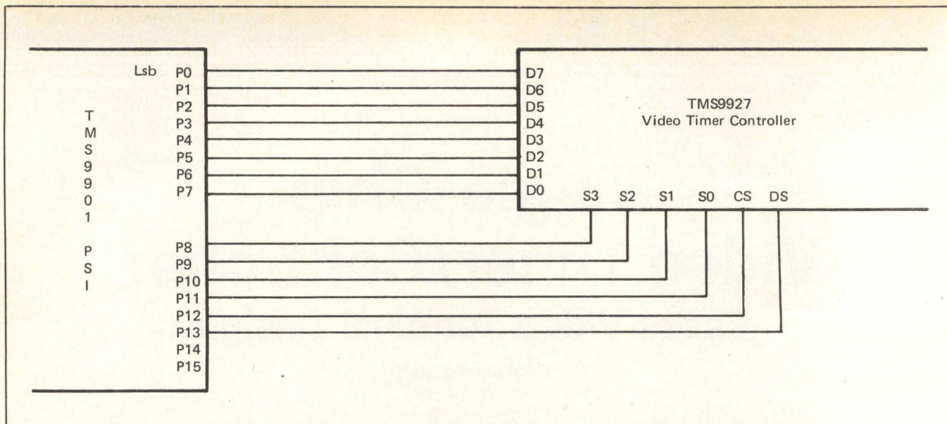
A 9927 signal timer + a 9901 interface + a video monitor = an high quality, stand-alone video terminal.
