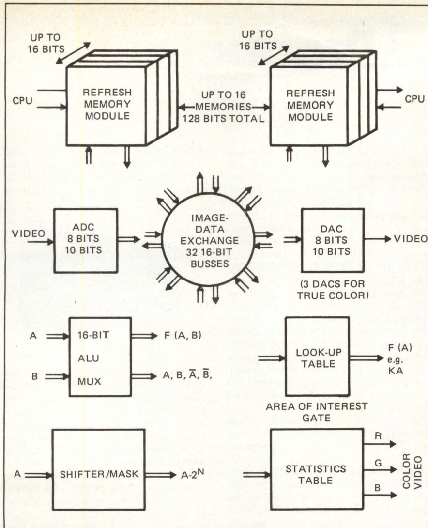
Figure 3: Image Processing Modules can be swapped by IDEX to form myriad architectures.
