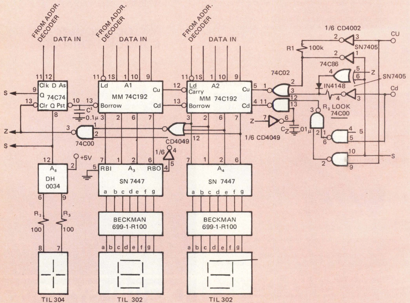
Up/Down Display Counter
