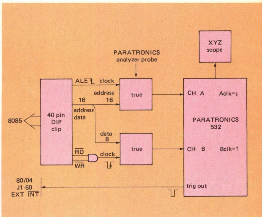
Figure 2: 80/04 connections
