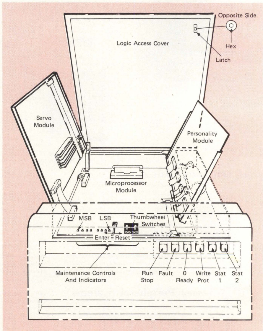
Hinged circuit module arrangement shows RM80 logic. Three main logic modules are accessible by lifting the logic access cover. The hinged module on the left-hand side is the servo module; the one on the right-hand side is the "personality module," used for interfacing to the controller, and the lowest is the microprocessor module. This arrangement enables repair personnel to reach the desired logic element rapidly and with a minimum of tools.
