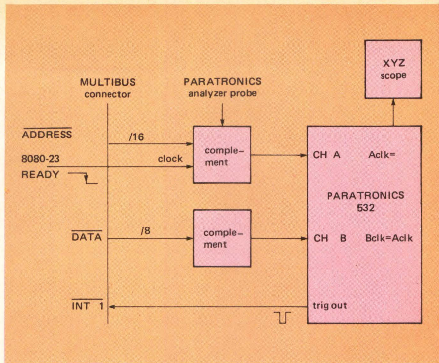
Figure 1: 80/10 connections
