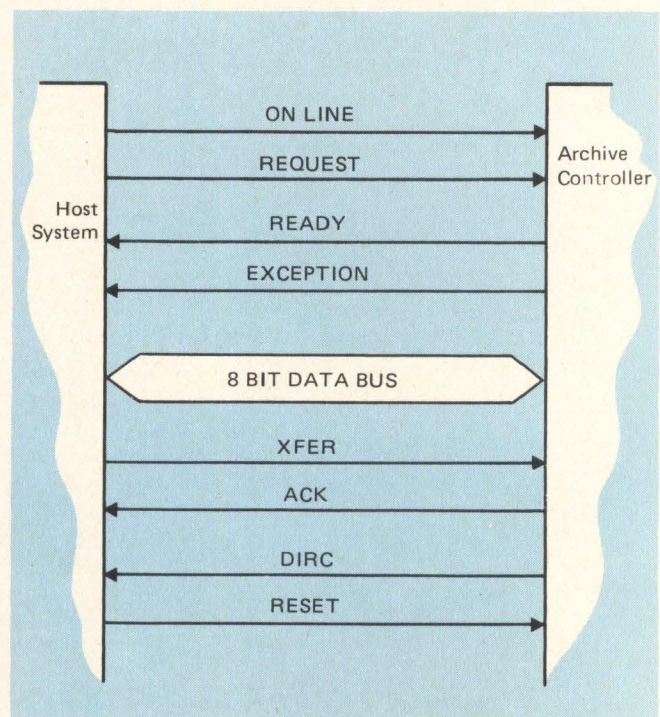
Controller commands for I/O and transfer.
