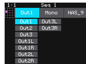
Output Selector
