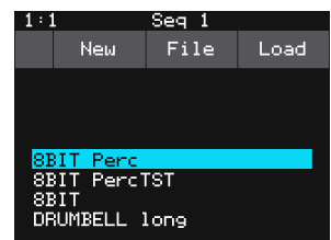
Preset Management
