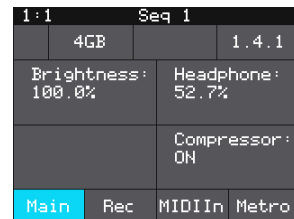
Tools Screen
