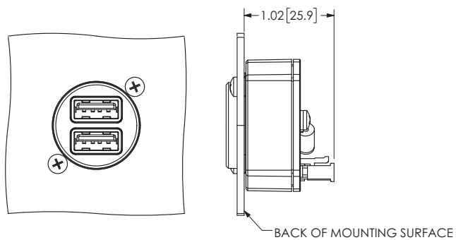
REAR CONNECTOR (-00/-20/-40 CONFIG), WITH CONNECTOR KIT (011-05044-00)
