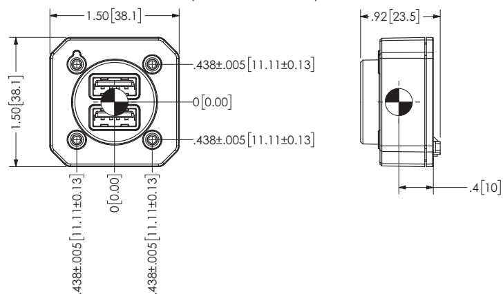
REAR CONNECTOR (-00/-20/-40 CONFIG), UNIT ONLY
