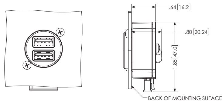
SIDE CONNECTOR (-01/-30/-50 CONFIG), WITH CONNECTOR KIT (011-05044-00)
