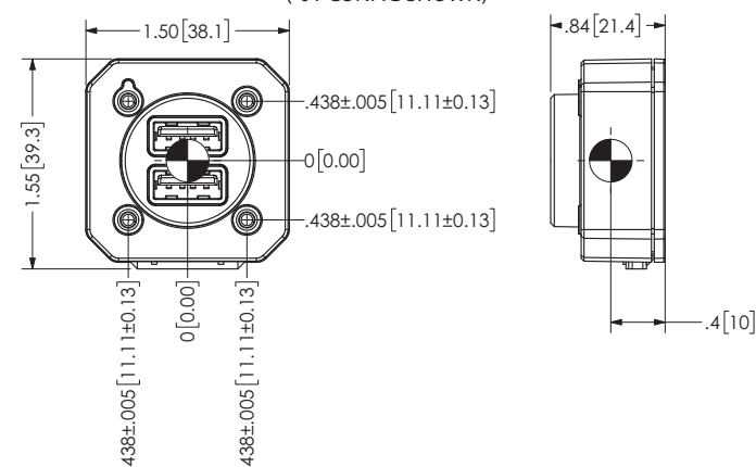
SIDE CONNECTOR (-01/-30/-50 CONFIG), UNIT ONLY
