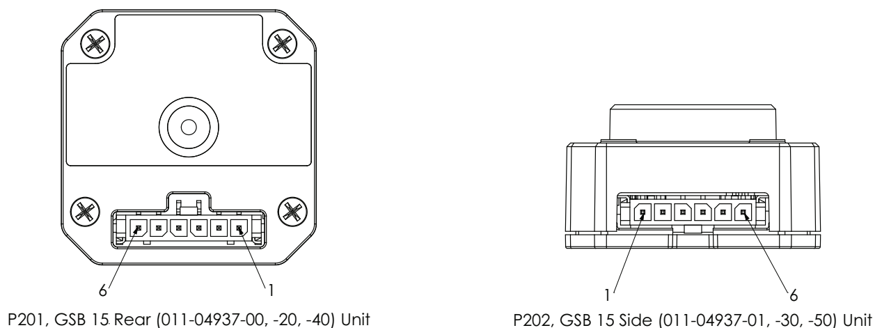
Figure 6-1. Unit View of P201/P202.
