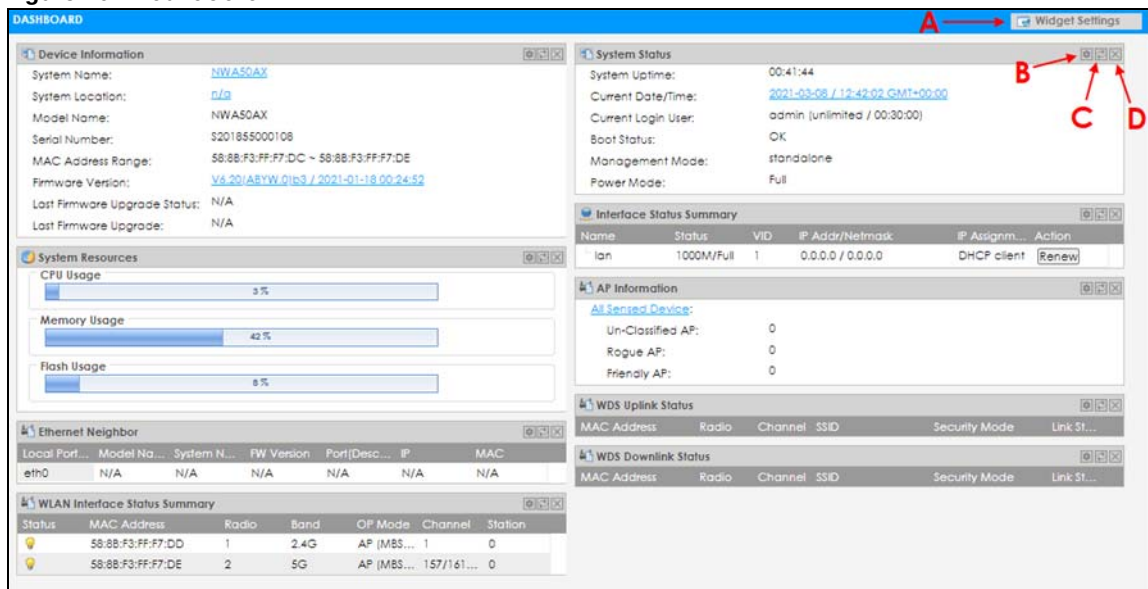
Figure 20 Dashboard
