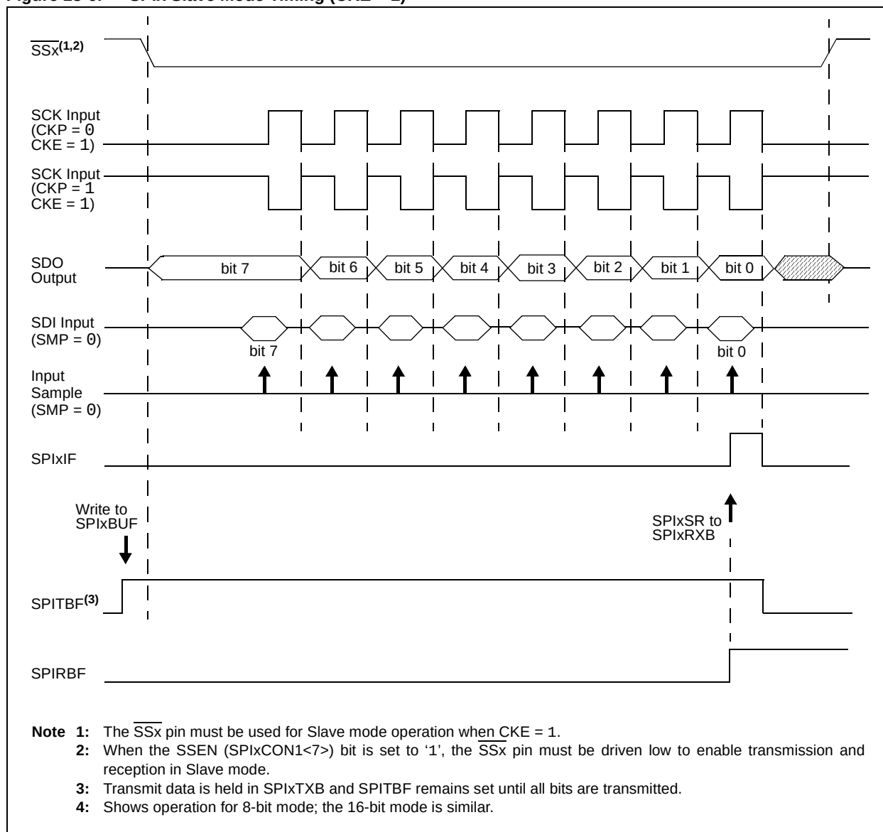
Figure 18-6: SPIx Slave Mode Timing (CKE = 1) (4)
