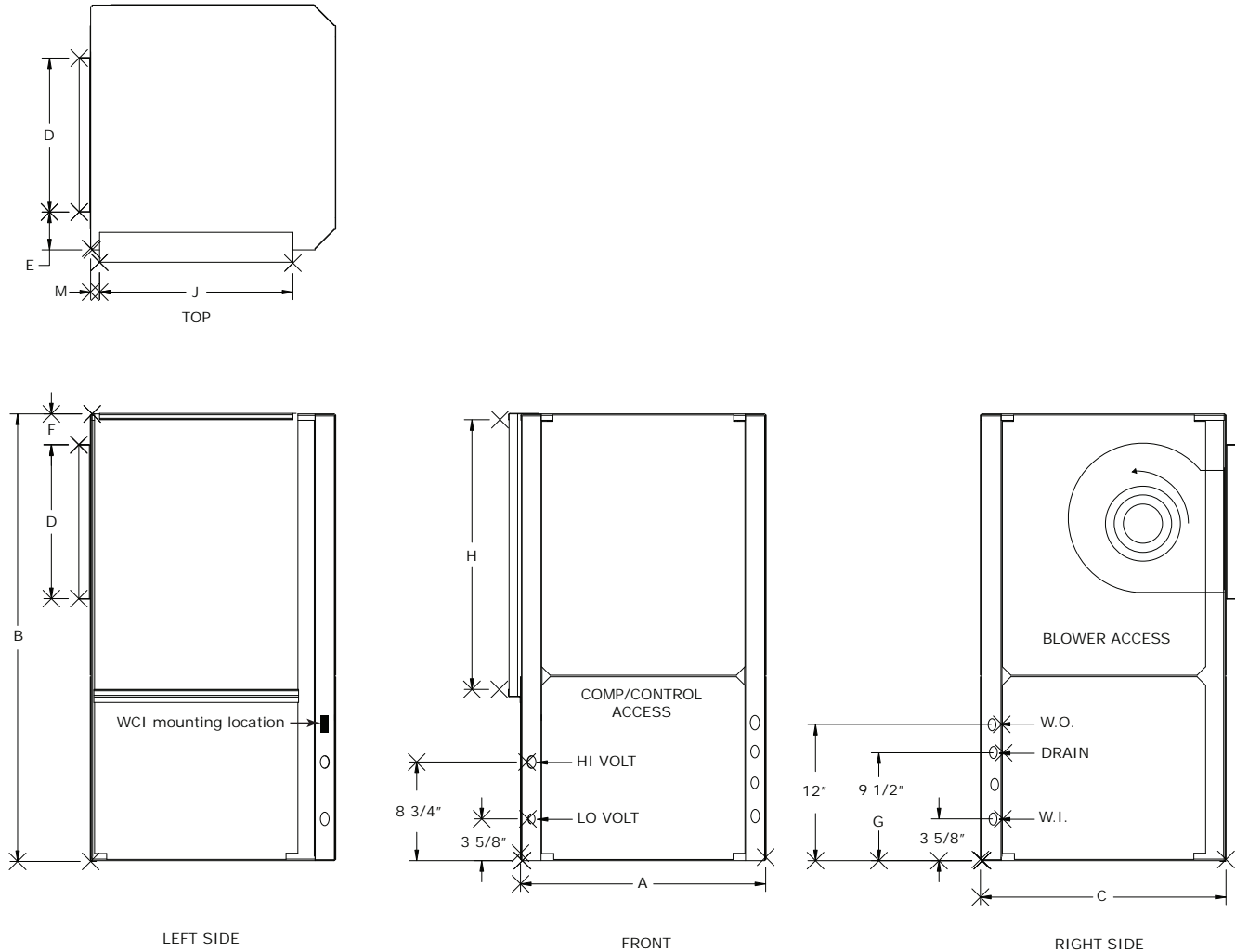
Figure 13. Left return/back supply VSV
