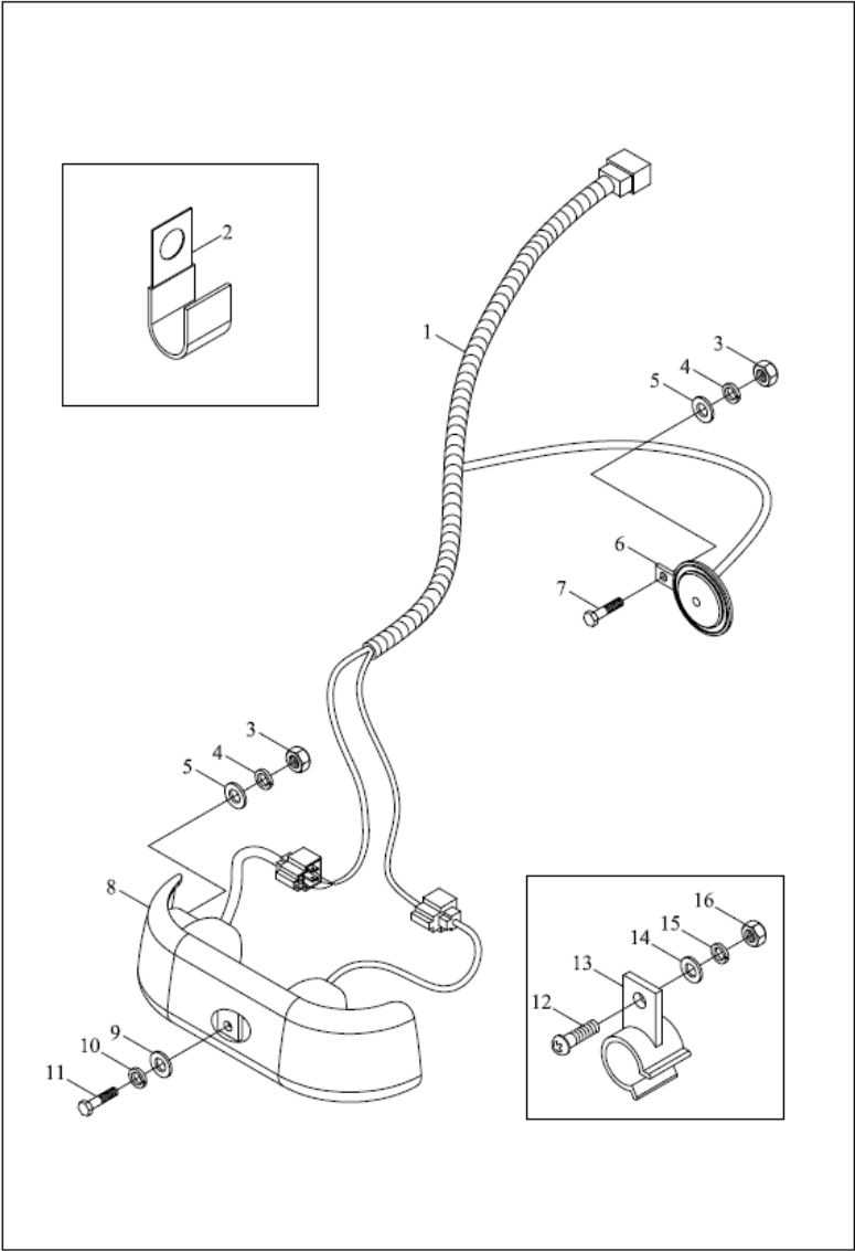
TB450.483B Front lamp wire harness mounting assembly
