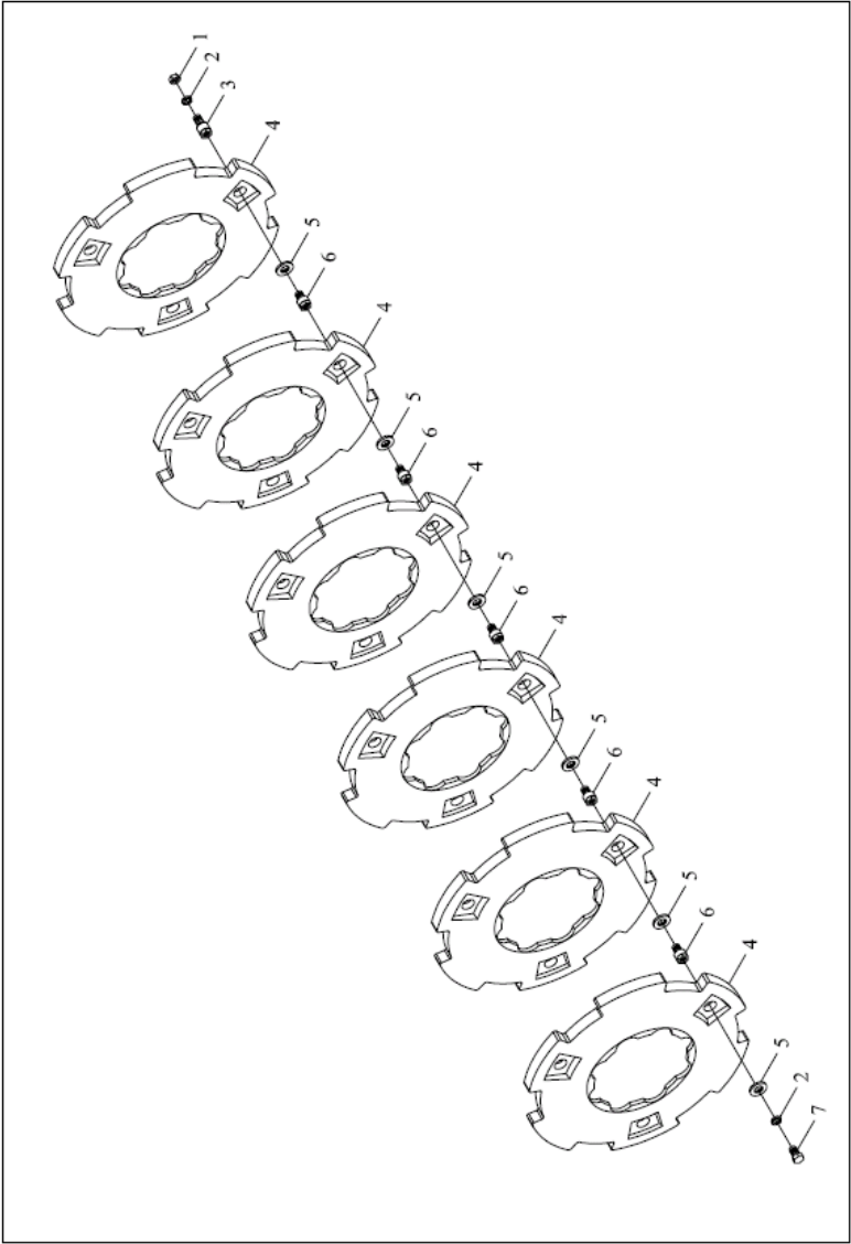
TB400.91Rear balance weight assembly
