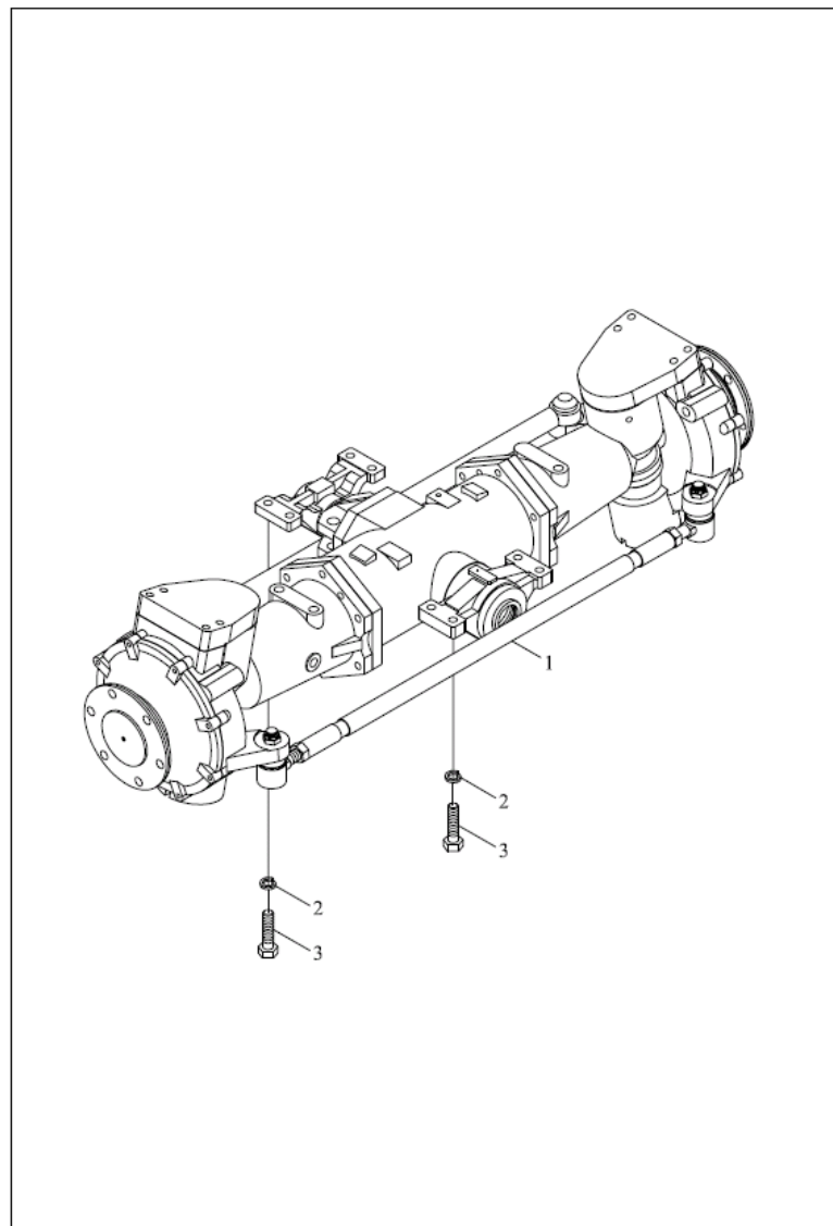
TB504.311 Front driving axle assembly-1
