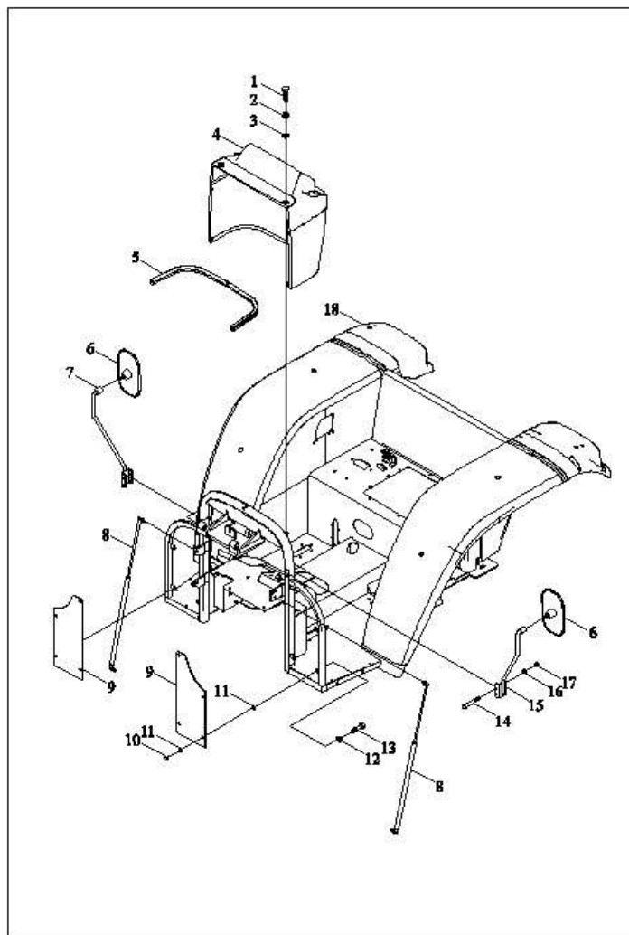
TB550.452U 地板总成-1
