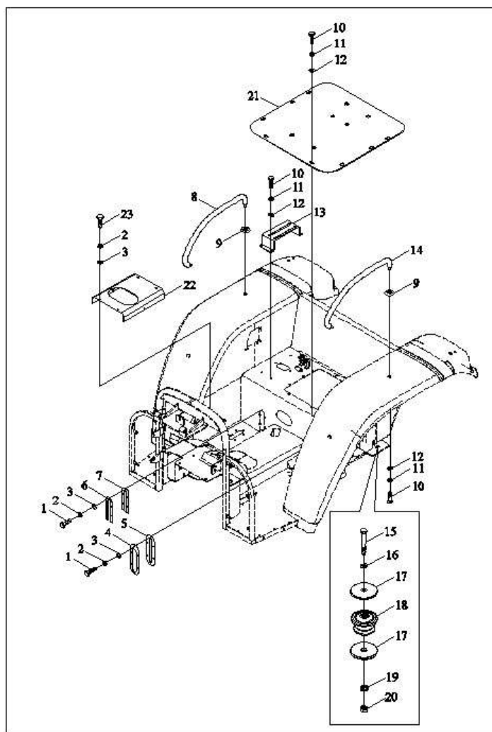
TB550.452U 地板总成-3
