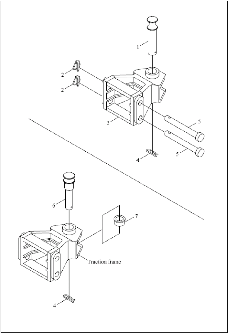
FT300.53.001Drag equipment assembly
