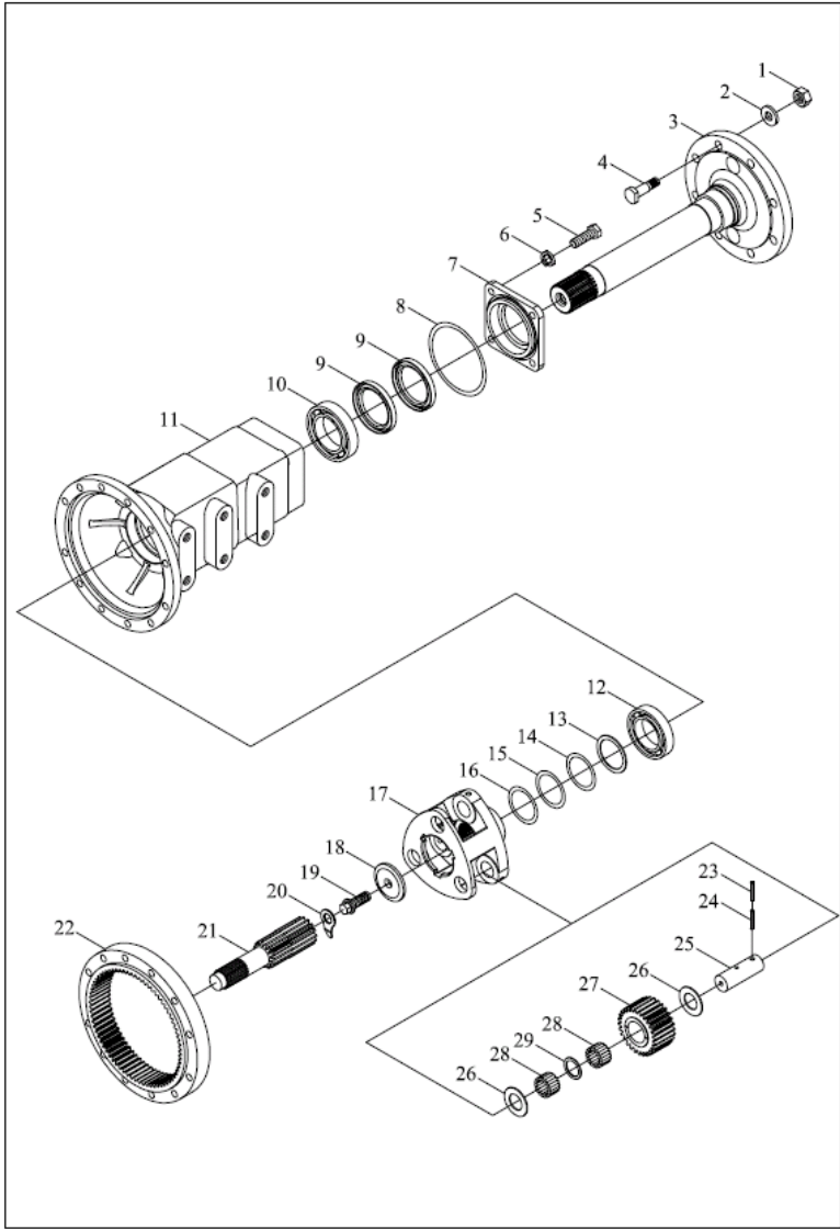
FT300.39.001 Final transmission assembly- -2
