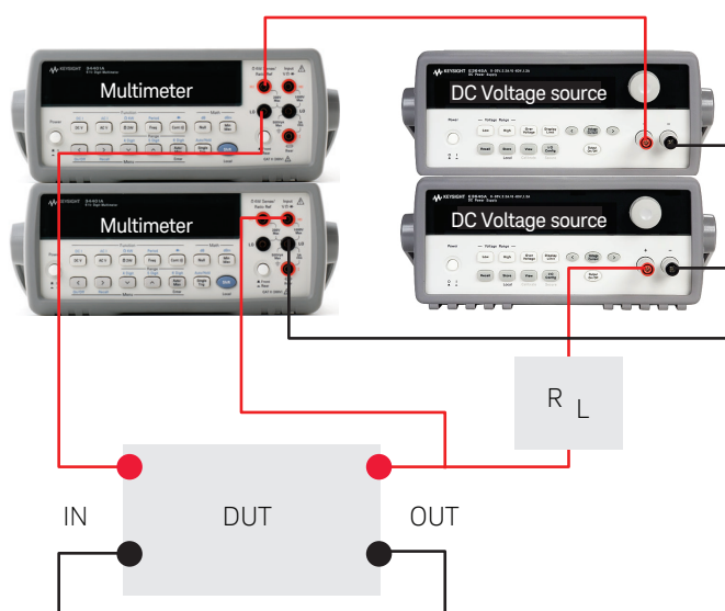
Bench-top setup example for 4-terminal DUT
