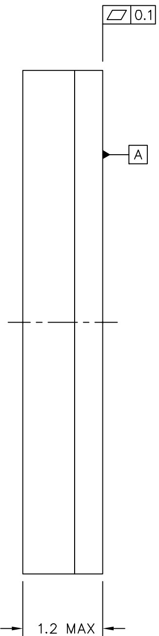
SIDE VIEW
