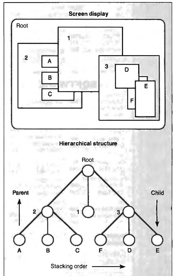
Figure 2: X Window treats overlapping windows as a hierarchy.
