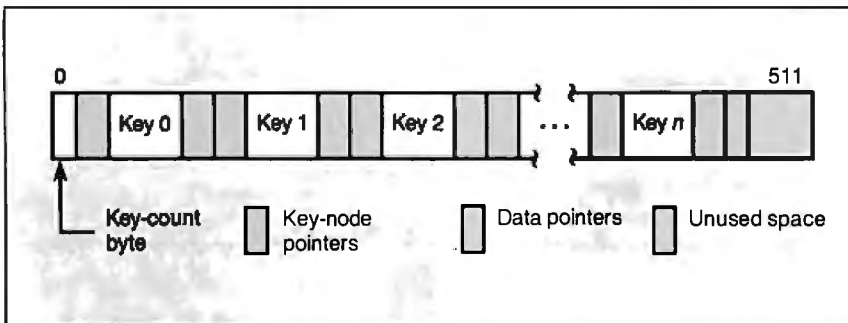
Figure 4: Format of a B-tree node. The node's length is deliberately set to 512 bytes, the usual size of a physical disk sector. The unused space at the right end of the node varies depending on key length (constant for a given key file) and the number of keys on the node.
