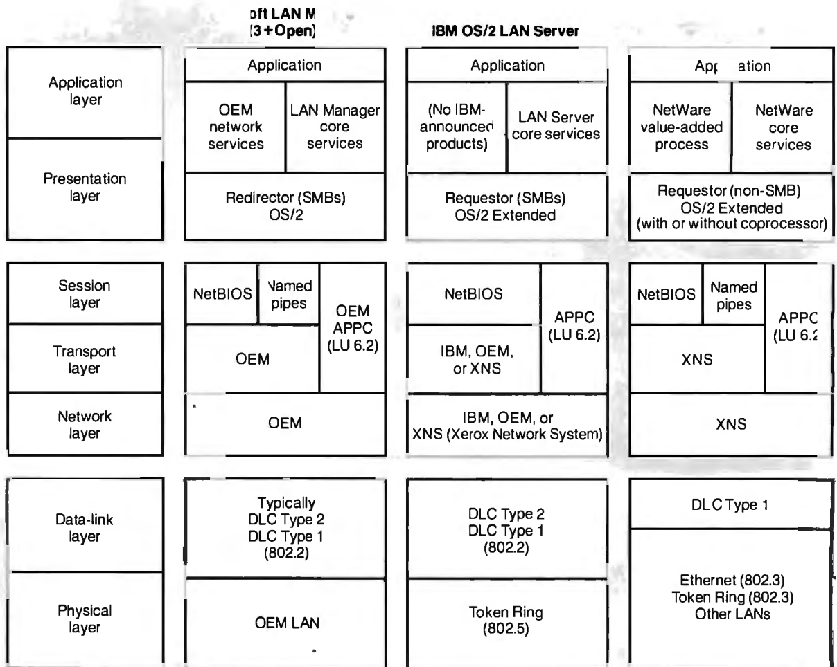
Figure 1: An Open Systems Interconnection and OS/2 architecture summary.
