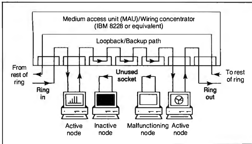
Figure 3: Signal flow in the medium access unit. Note that any or all nodes in the star-wired ring can be bypassed if necessary.
