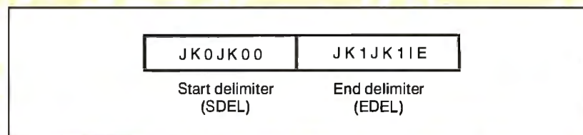
Figure D: The abort delimiter consists of a start delimiter and an end delimiter together.
