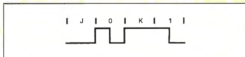
Figure C: Manchester code violations.
