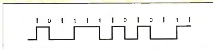
Figure B: Differential Manchester encoding.
