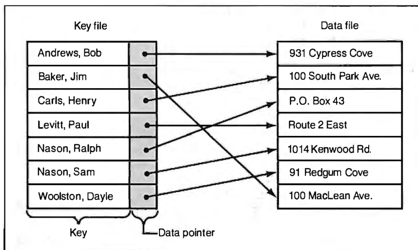
Figure 1: A super-simple KFS. The key file holds keys and attached data pointers. Each data pointer is an offset into the data file where the associated data is located.
