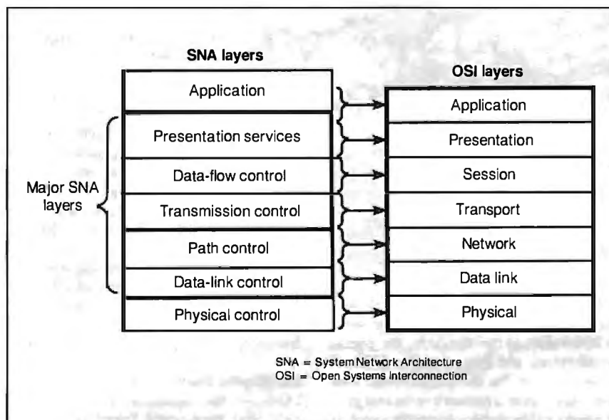
Figure 1: The SNA layers versus the OSI layers. While the correspondences are very close, they are not exact.
