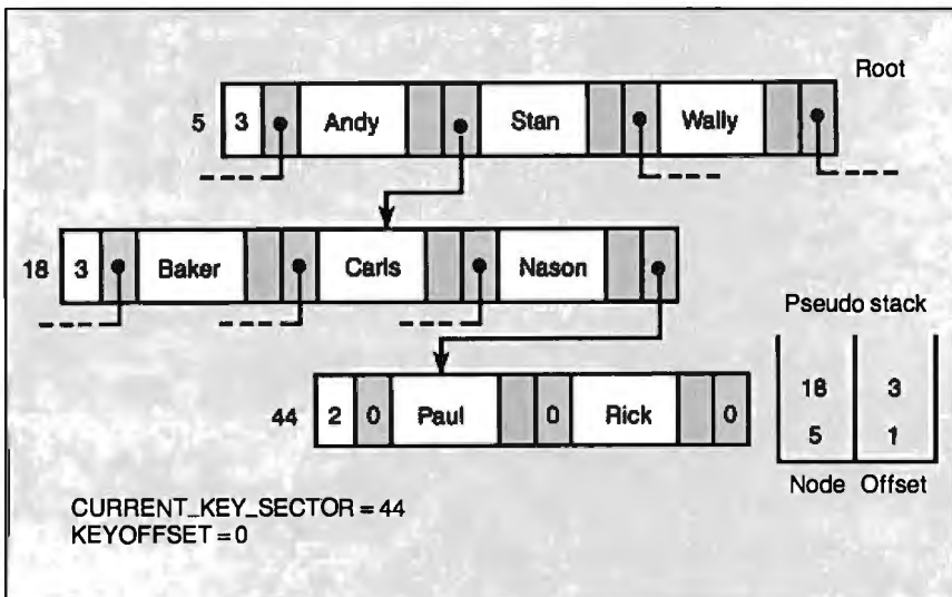
Figure 6: SEEK_KEY searches for the key PAUL in this example. As the routine moves down the tree, it records its trail on the pseudo stack. SEEK_KEY leaves CURRENT_KEY_SECTOR set to the target node and KEYOFFSET set to the key number within the node.
