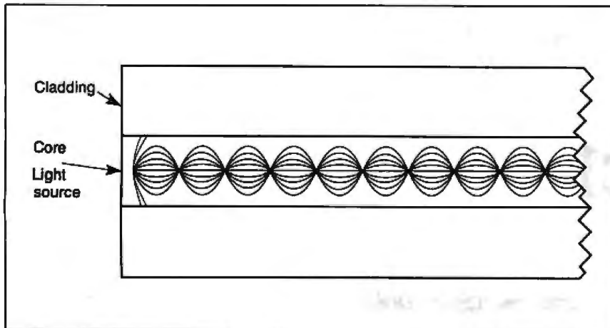
Figure 1: With graded-index multimode fiber cable, light is constantly refocused as it travels through the core.
