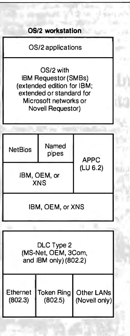
Figure 2: The Banyan VINES and OS/2 workstation architectures.
