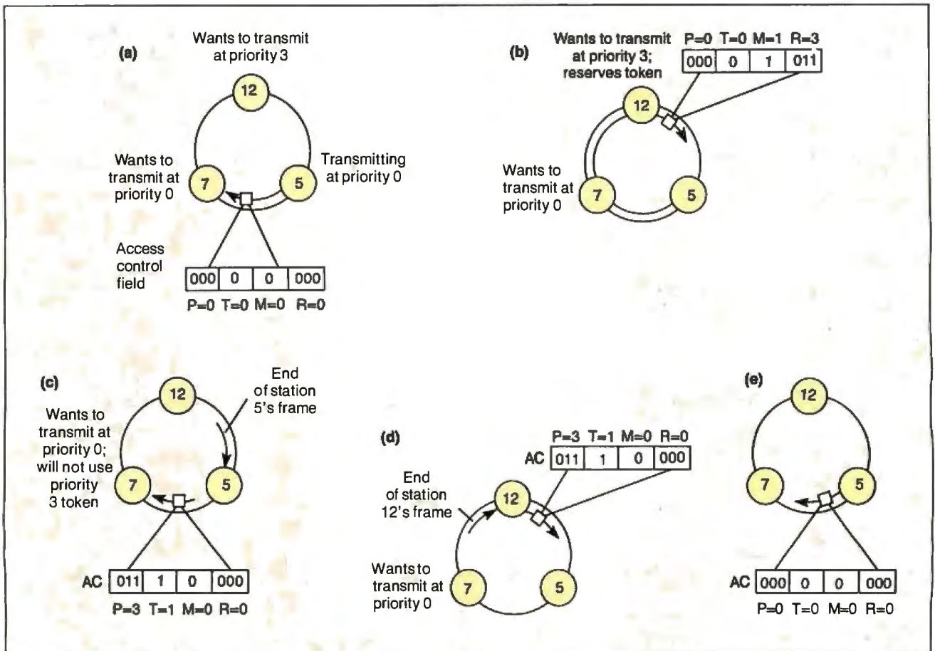
Figure 5: Placing a reservation. (a) Station 5 is transmitting a frame to station 7 on the ring. Normally, station 7 would be the next node to get the token, even though station 12 had a higher-priority frame to transmit. (b) Station 12 sees that the reservation field of the frame is less than 3 and places a 3 there. The frame continues back to station 5, which absorbs the frame and emits a token. (c) The token emitted by station 5 had priority 3, so station 7 does not use it. The token continues on to station 12, which uses the token to transmit a frame. (d) When station 12 has finished transmitting, it releases a token, still at priority level 3. (e) Station 5 receives a token at priority level 3 and "remembers" that it was the one to raise the priority of the token. It therefore restores the priority to 0 so that station 7 will have a chance to transmit.
