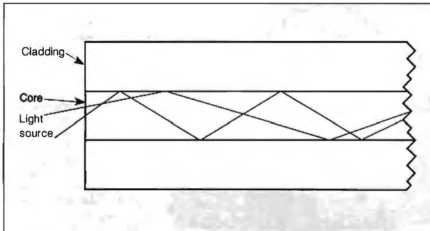
Figure 2: In step-index multimode fiber, light travels through the fiber, being refracted back and forth from the core's boundary with the cladding.
