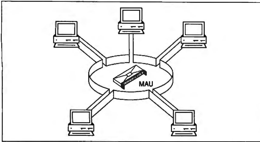
Figure 2: At the lowest level, the physical layer, a Token Ring looks like a star (hence the term "star-wired ring topology") in which each node is connected to a wiring concentrator, the medium access unit.
