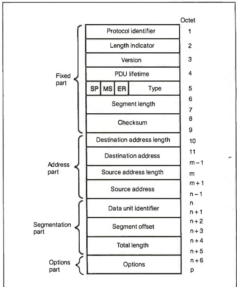
Figure A: The 15-part header format for the ISO-IP, the ISO's standard for an internet protocol.
