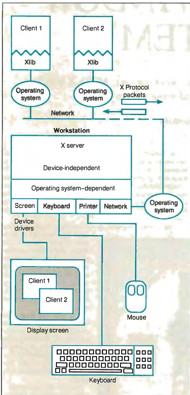
Figure 1: The client program sends packets of instructions to the server, which contains the hardware-dependent drivers for that workstation. An X server controls not only the screen but also the keyboard and a pointing device with up to five buttons.
