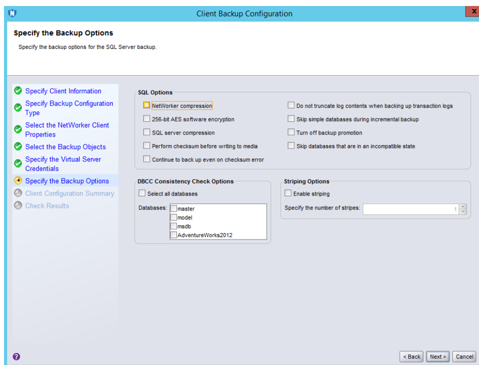
Figure 16 Specify the Backup Options page
