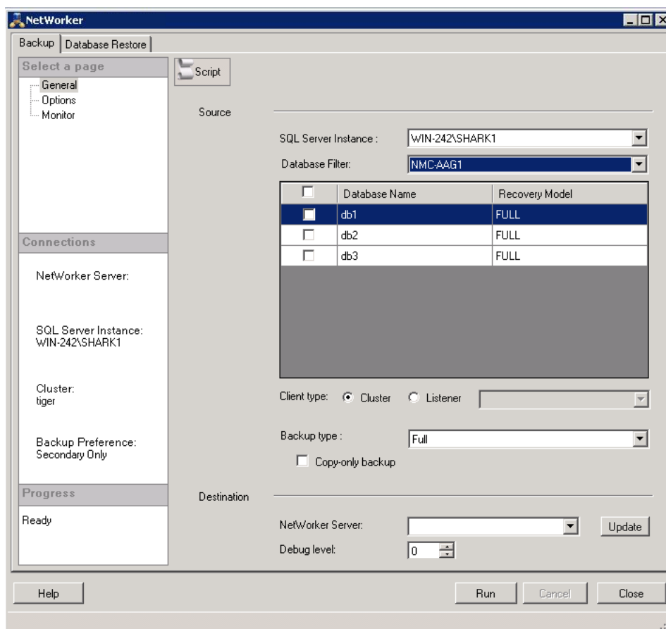
Figure 10 NetWorker Backup General page
