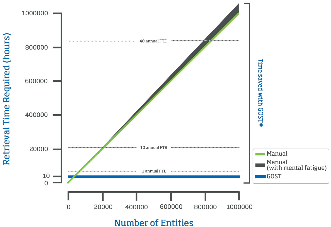
Figure 2) Retrieval time comparison between a manual review process using Google, and a semi-automated process using GOST.
