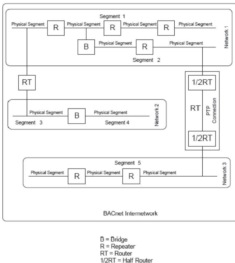
Figura 34 – BACnet Internetwork
