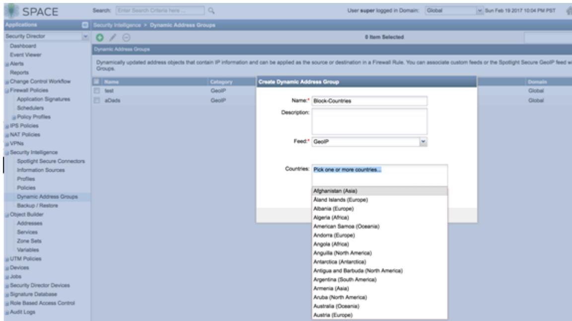
Figure 107: Spotlight Secure: Create Geo IP with Dynamic Address Group
