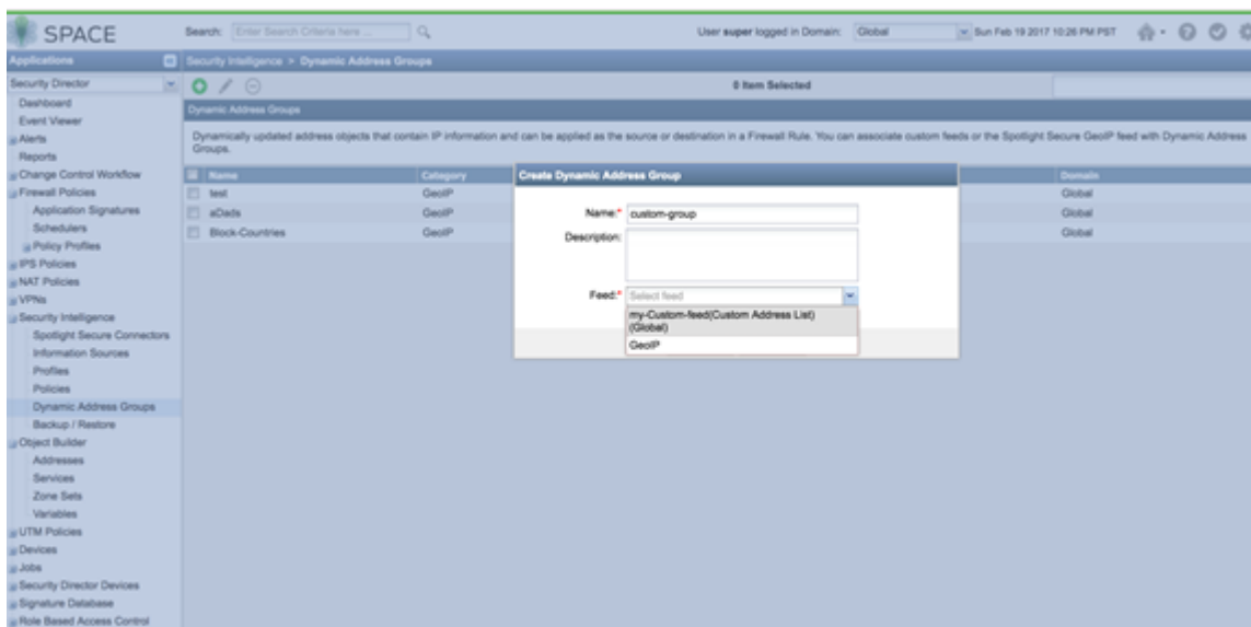
Figure 101: Spotlight Secure: Select Custom Feed in Dynamic Address Group
