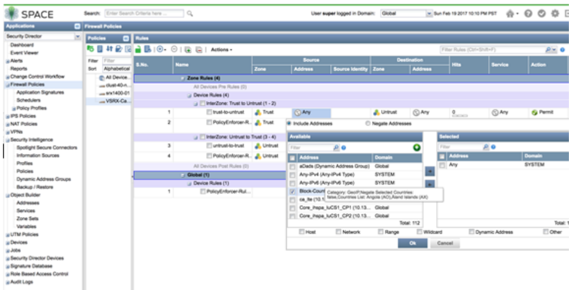
Figure 108: Spotlight Secure: Use Geo IP in Firewall Policy
