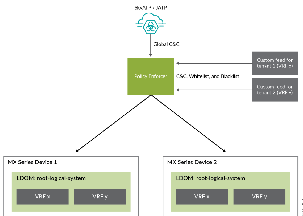
Figure 72: LSYS and VRF Instance Support
