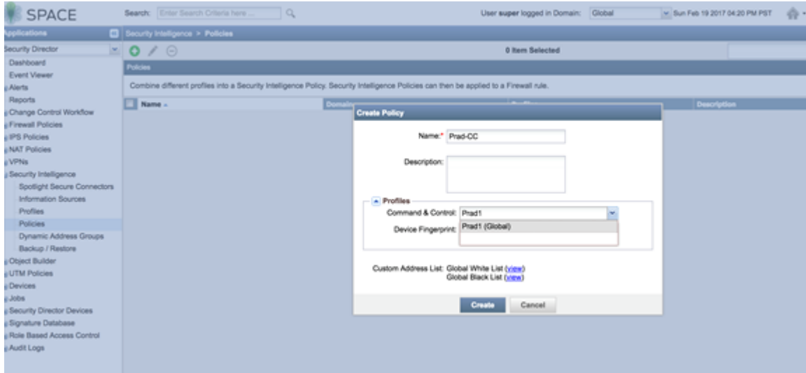
Figure 92: Spotlight Secure: Create Security Intelligence Policy
