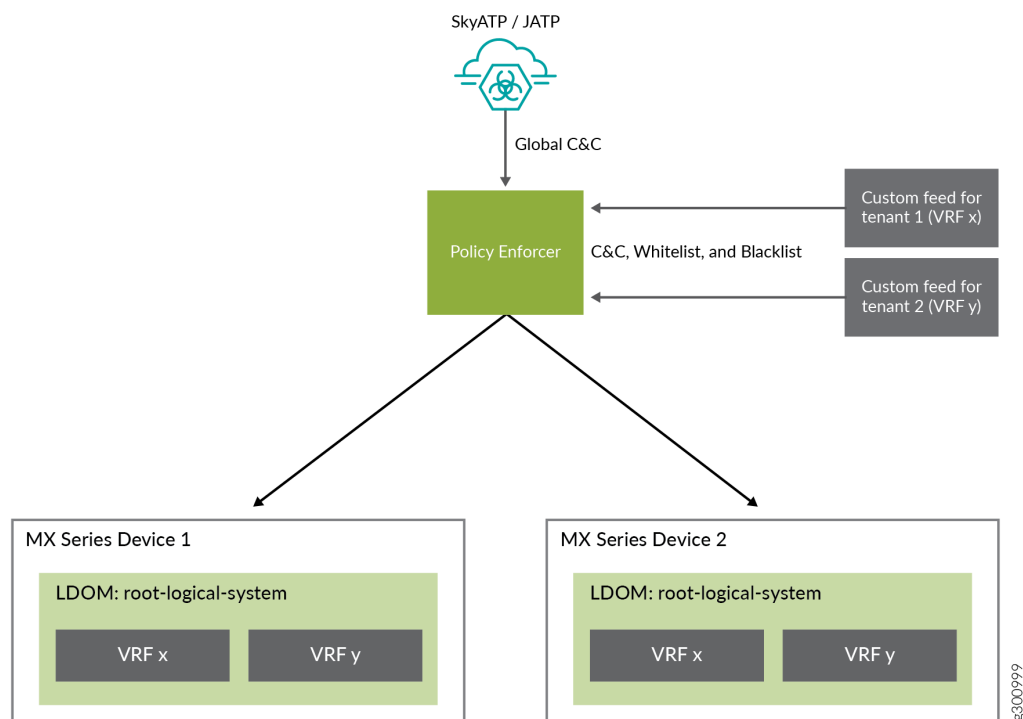
Figure 73: LSYS and VRF Instance Support
