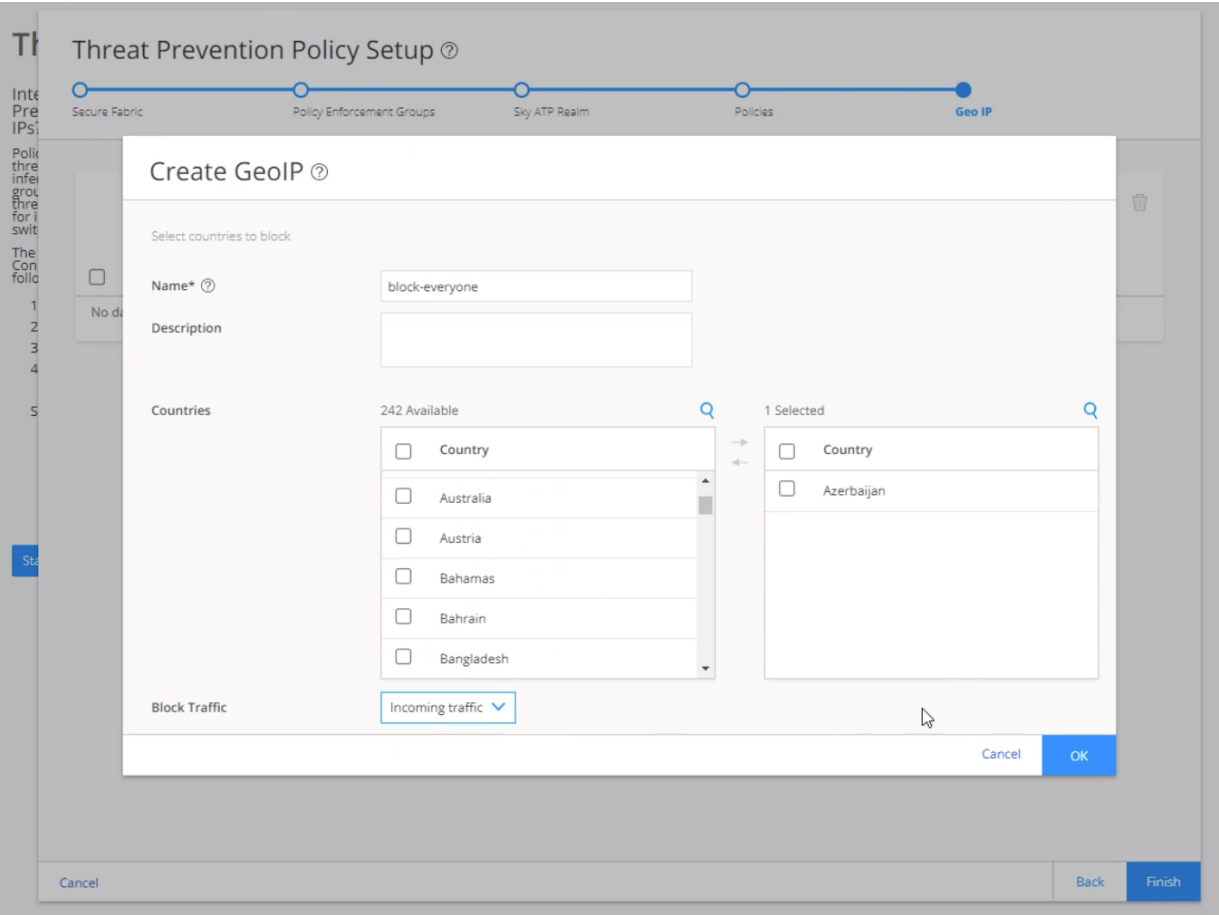
Figure 71: Create Geo IP
