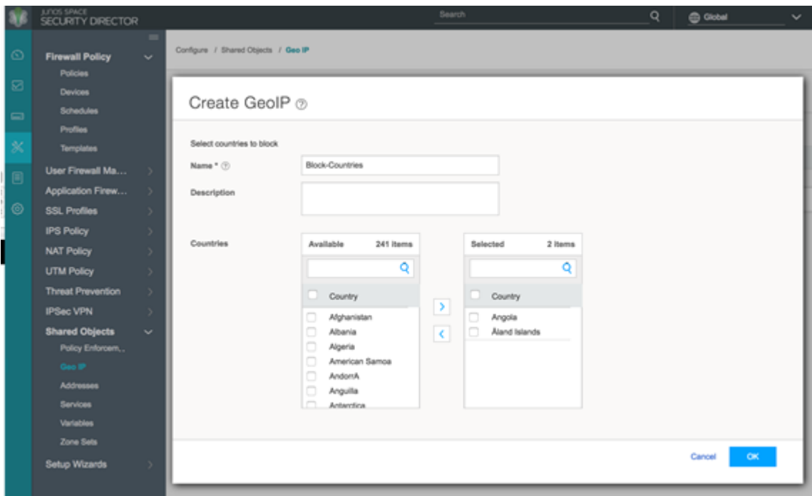
Figure 109: Policy Enforcer: Create Geo IP
