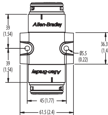
Double-sided Base
