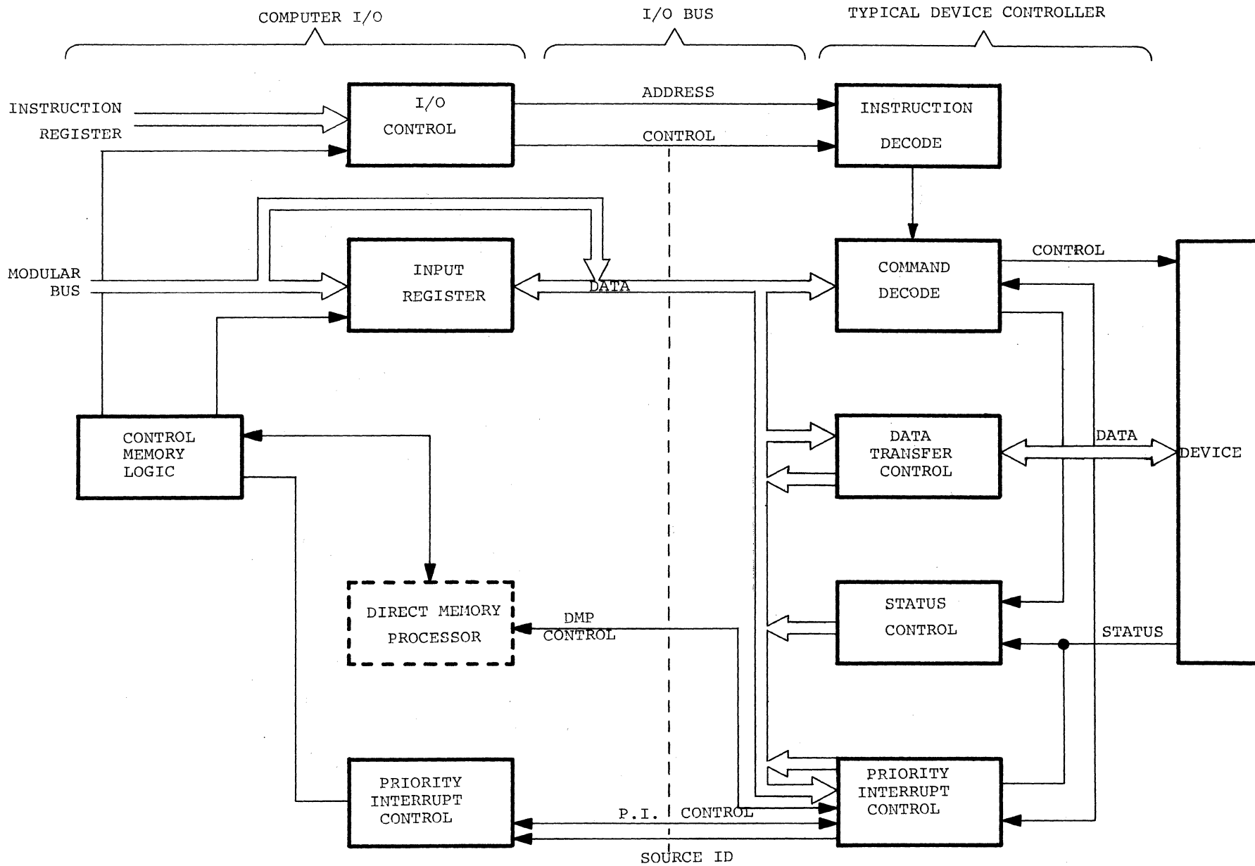
FIGURE 5-1 INPUT/OUTPUT SUBSYSTEM BLOCK DIAGRAM
