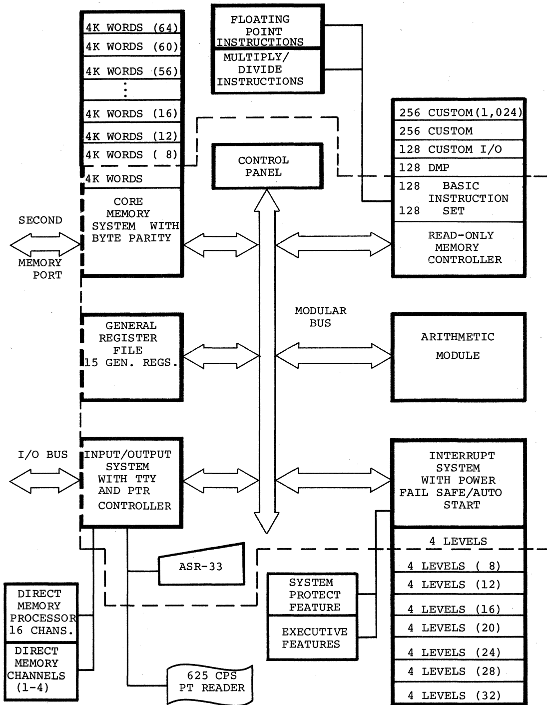
Figure 1-1 MODCOMP III Block Diagram
