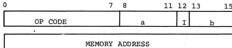
Two Word Format
