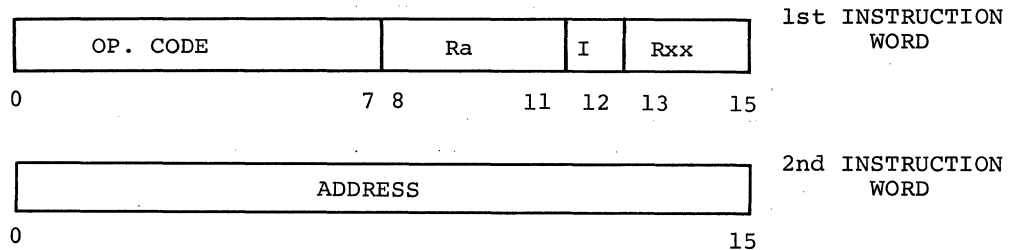
BASIC MEMORY ADDRESS FORMAT
