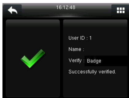
Verification Succeeds.
