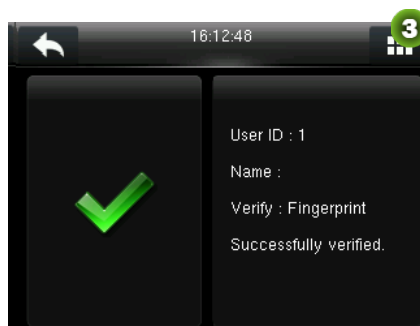
Verification Succeeds.
