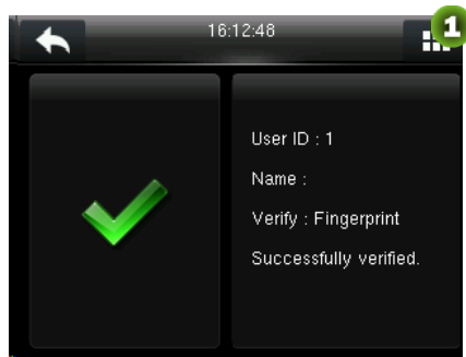
Verification Succeeds.
