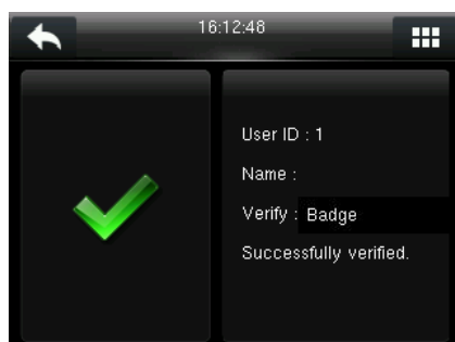
Verification Succeeds
