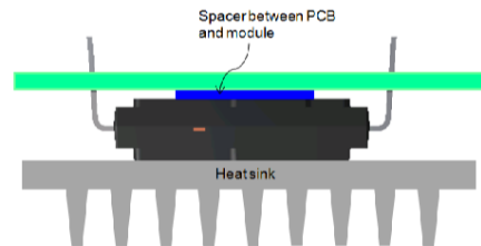
Figure 11. Examples of the Spacer Type
