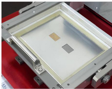
Aligning and positioning of the screen mask to the module DBC area
