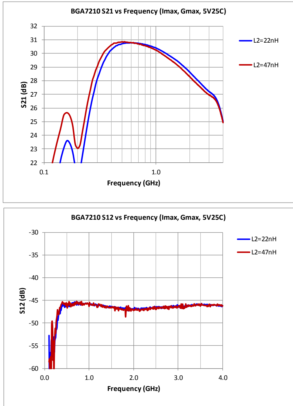
Fig 2. Comparison S21 and S12 for Two RF Choke L2 Values (Imax, Gmax)
