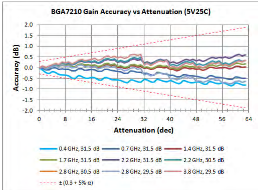
Fig 5. Gain Accuracy vs. Attenuation Setting, L2=47 nH
