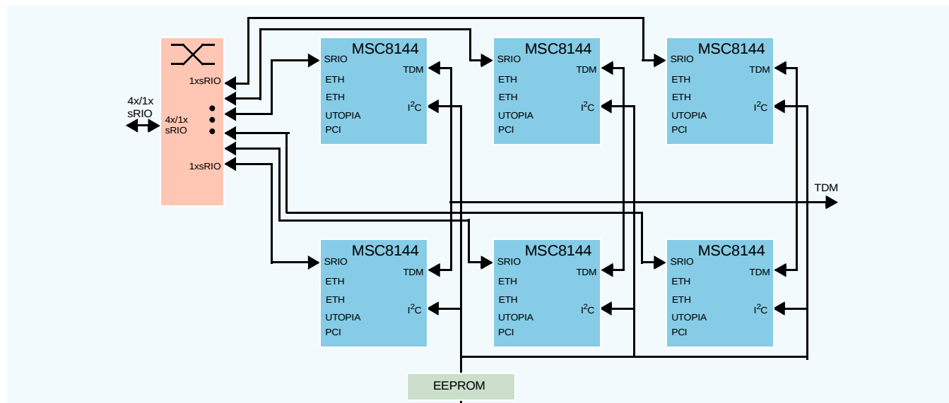
Figure 4. SerDes Connectivity
