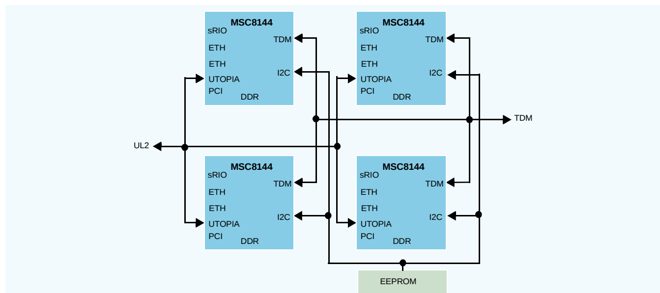
Figure 2. DSP Farm Example Using UTOPIA and TDM
