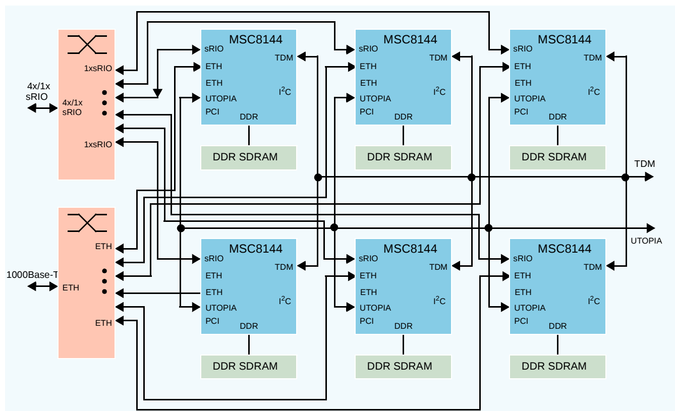
Figure 1. Generic System Block Diagram
