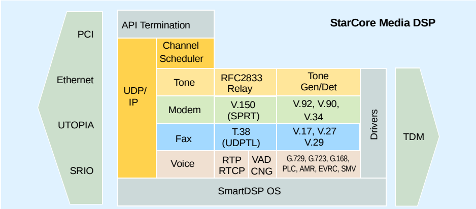
Figure 7. Application Software Model
