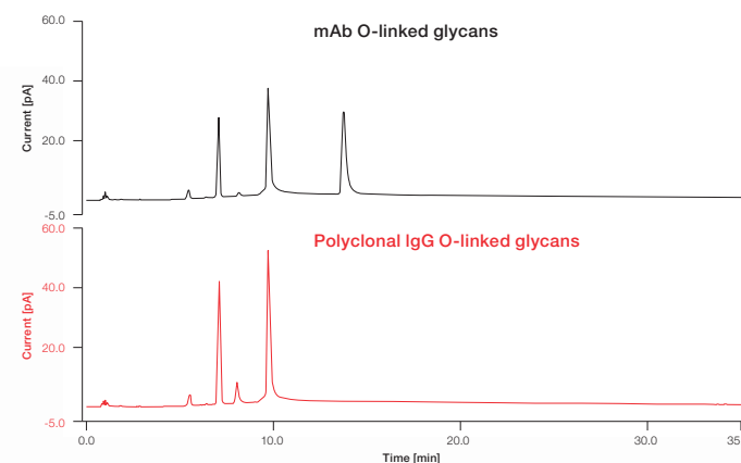
Direct and accurate quantitation of O-linked glycans using LC-CAD
