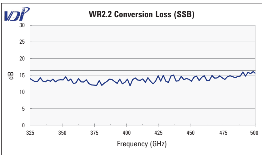
Figure 7. Measured intrinsic mixer conversion loss for the N9029AV02 (325 to 500 GHz) frequency extension module.
