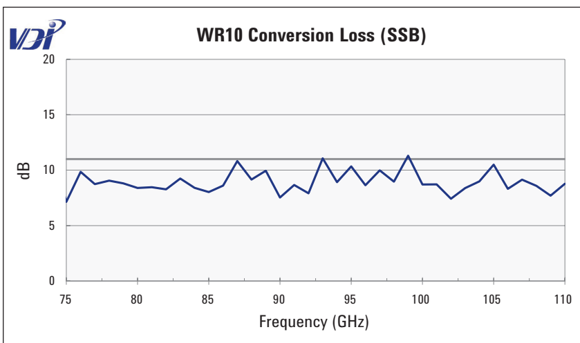
Figure 12. Measured intrinsic mixer conversion loss for the N9029AV10 (75 to 110 GHz) frequency extension module.
