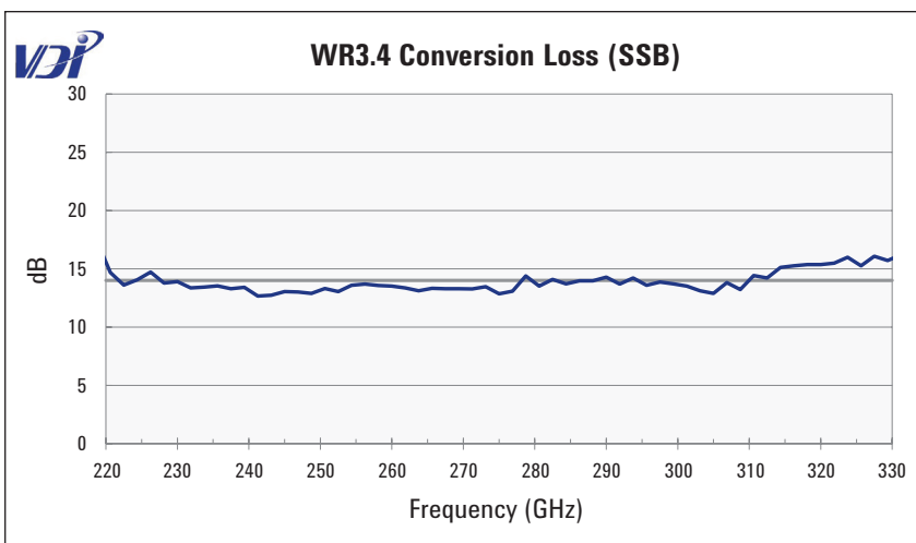
Figure 8. Measured intrinsic mixer conversion loss for the N9029AV03 (220 to 330 GHz) frequency extension module.
