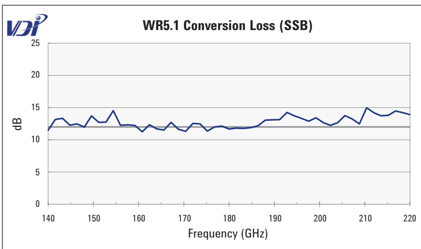
Figure 9. Measured intrinsic mixer conversion loss for the N9029AV05 (140 to 220 GHz) frequency extension module.
