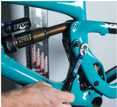
18. Using a 5mm allen wrench, thread both collet bolts into the pivot axles. Finish tightening using a properly calibrated torque wrench.
