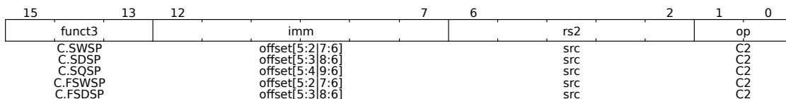
Figure 50: Stack-Pointed-Based Stores
