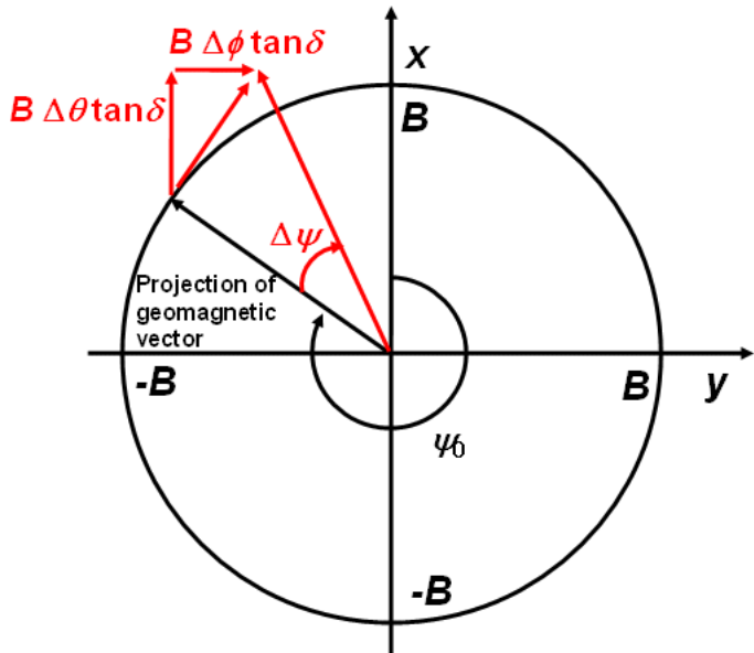
Figure 4. Geometry of Accelerometer-Induced Compass Angle Errors
