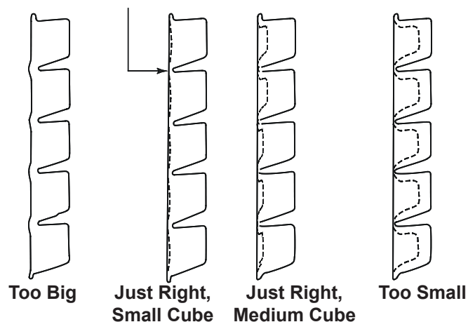
Ice Bridge Thickness Measurement
