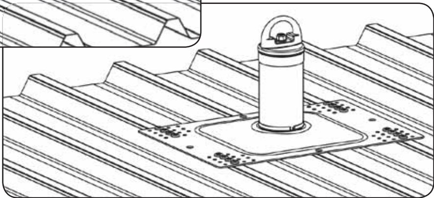
Fig. 8c - Completely Installed
